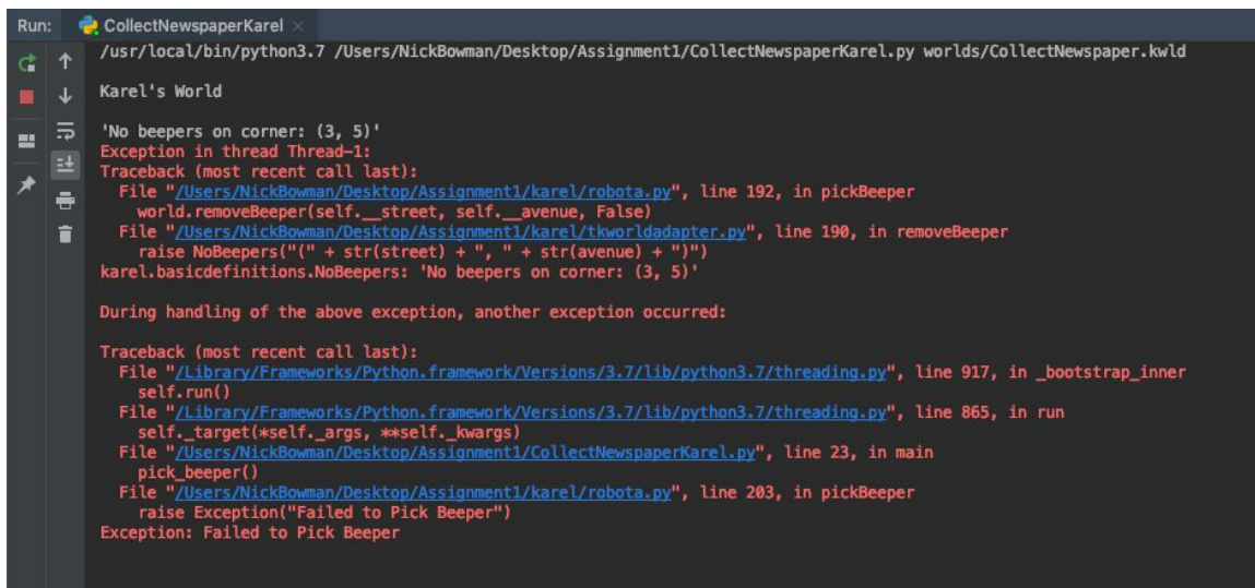
Figure 9: The bottom panel of PyCharm displays an error message that occurs when something has gone wrong in Karel's world
