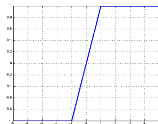
Figure 11: The response of a hard tanh nonlinearity
