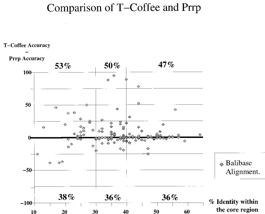
Figure 3. Comparison between T-Coffee and Prpp. For each alignment in BaliBase, the average level of pair-wise identity was measured on the core regions of the reference alignment. Alignment accuracy was assessed for T-Coffee and Prpp on these core regions. The latter two values were subtracted (%T-Coffee accuracy – %Prpp accuracy) and plotted versus the average identity for the alignment. Points in the top area indicate alignments where T-Coffee is outperforming Prpp and inversely for the bottom area. Alignments have been divided into three sets: below 30% identity (34 alignments), between 30 and 40% identity (52 alignments) and above 40% identity (55 alignments). The percentages given in the corners of the plot indicate the fraction of alignments for which T-Coffee outperforms Prpp (top) and vice-versa (bottom). These percentages do not add up to one hundred as for some alignments the same accuracy was obtained with each method (e.g. for alignments having less than 30% identity, T-Coffee outperforms Prpp in 53% of the cases, Prpp outperforms T-Coffee in 38% of the cases, and the two methods draw in 9% of the cases).
