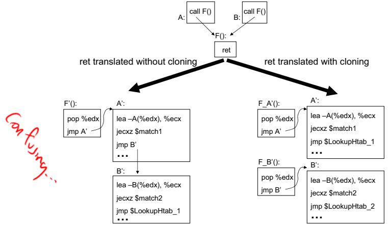
Figure 3. Compiling indirect jumps and returns
