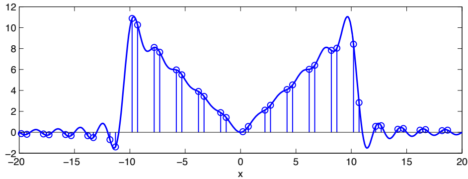
Figure 3: Bunched samples, and the original sinc interpolation. Note that we've completely missed the peak ripple on the right.
