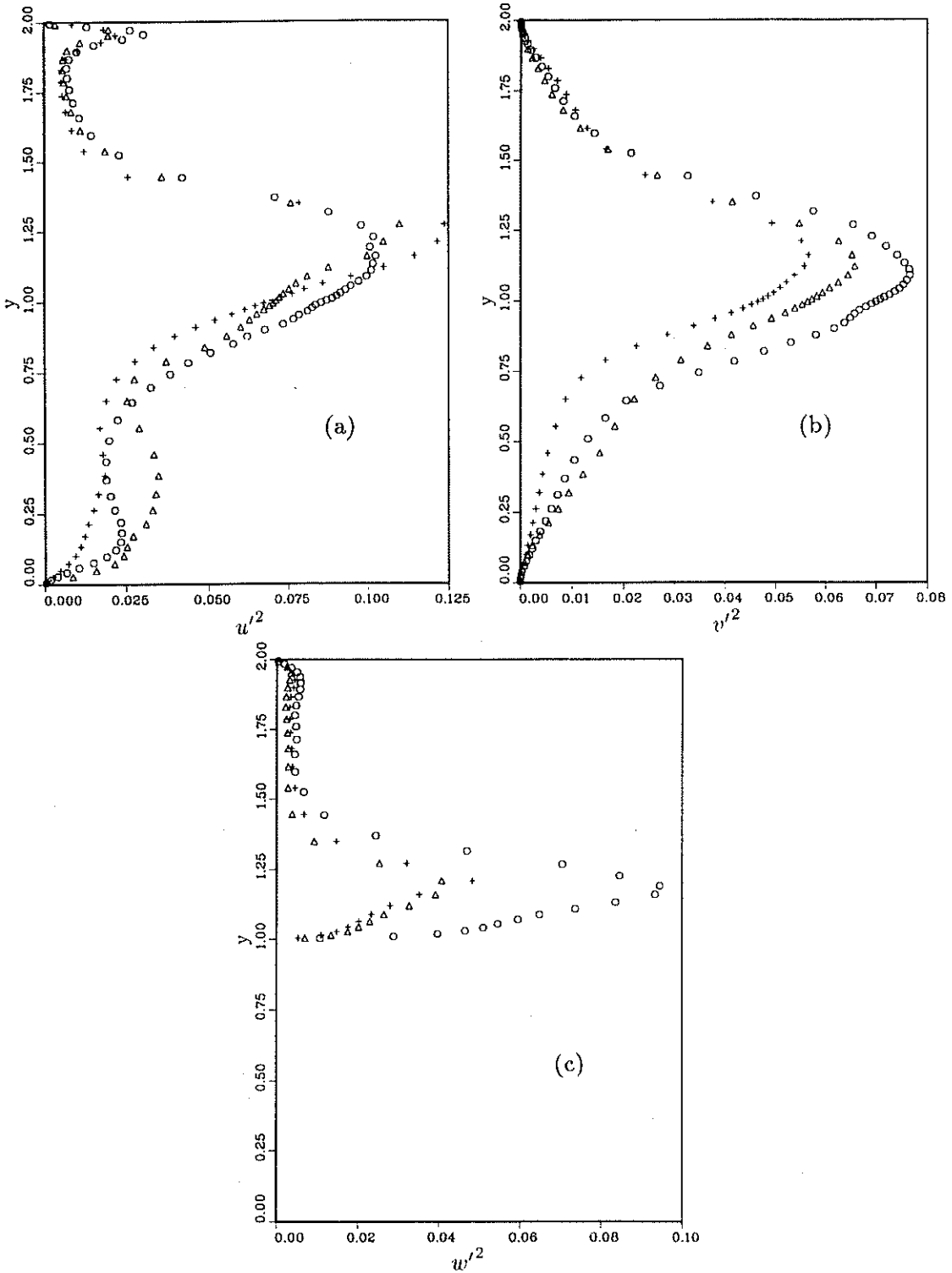
FIGURE 5. Averaged turbulent fluctuation profiles; (a) streamwise ( u'^2 ) at x=12 , (b) normal ( v'^2 ) at x=12 , (c) spanwise ( w'^2 ) at x=11 : o, DNS; \Delta , LES with DSGM; +, LES with C_s=0.01 .
