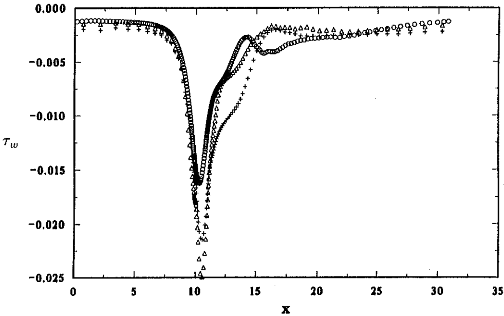
FIGURE 3(b). Averaged wall shear stress at the upper wall: \circ , DNS; \triangle , LES with DSGSM; + , LES with C_s=0.01 .
