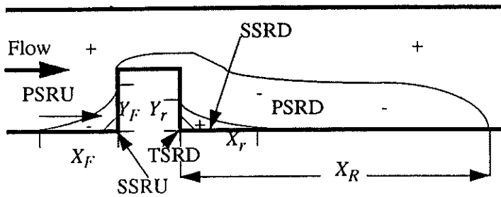
FIGURE 2. Schematic drawing of SR regions.
