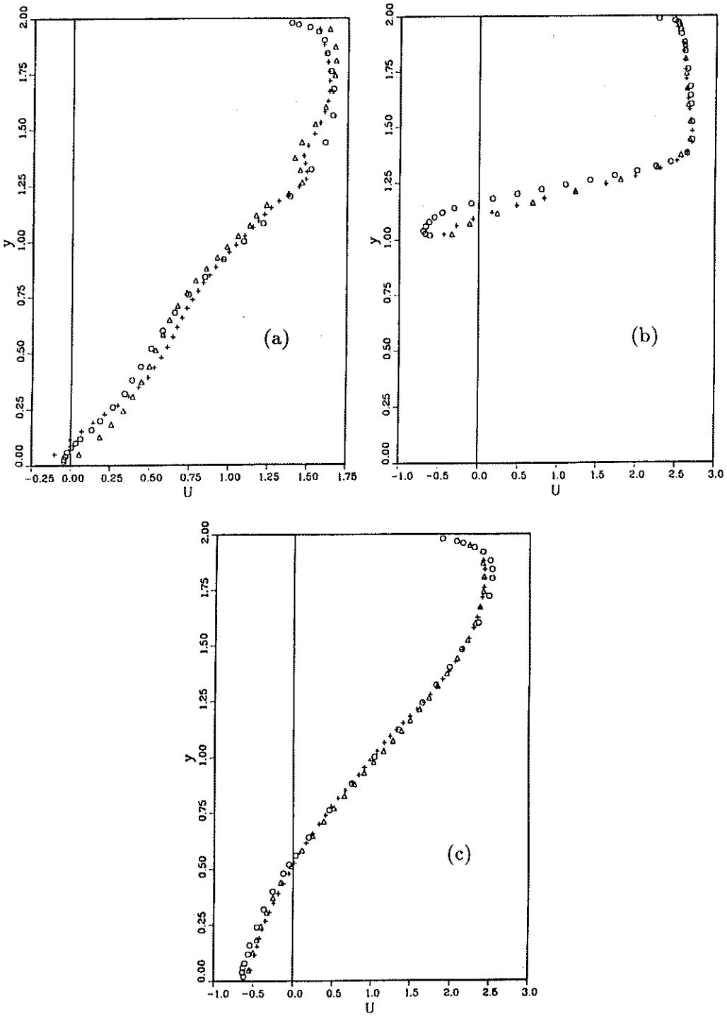
FIGURE 9. Streamwise velocity profiles: (a) x=9.6 , (b) x=10.8 , (c) x=15 : o, exp.; \Delta , 96x32x32; +, 128x48x40.
