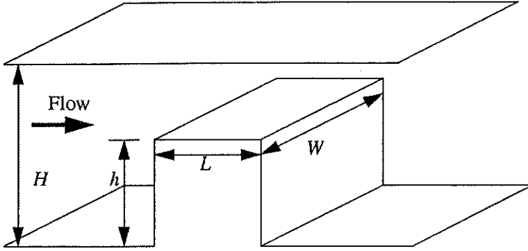
FIGURE 1. Physical configuration.
