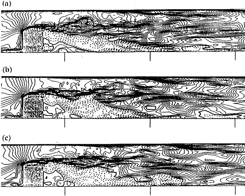
FIGURE 7. Regions of instantaneous negative u ; solid, positive; dash, negative; thick solid, 0; increment, 0.016: (a) t=0 ; (b) t=\Delta t ; (c) t=2\Delta t .
