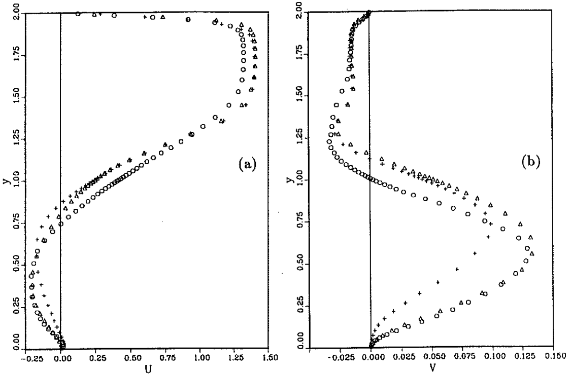
FIGURE 4. Averaged velocity profiles at x=12 ; (a) streamwise ( U ), (b) normal ( V ): \circ , DNS; \triangle , LES with DSGSM; + , LES with C_s=0.01 .
