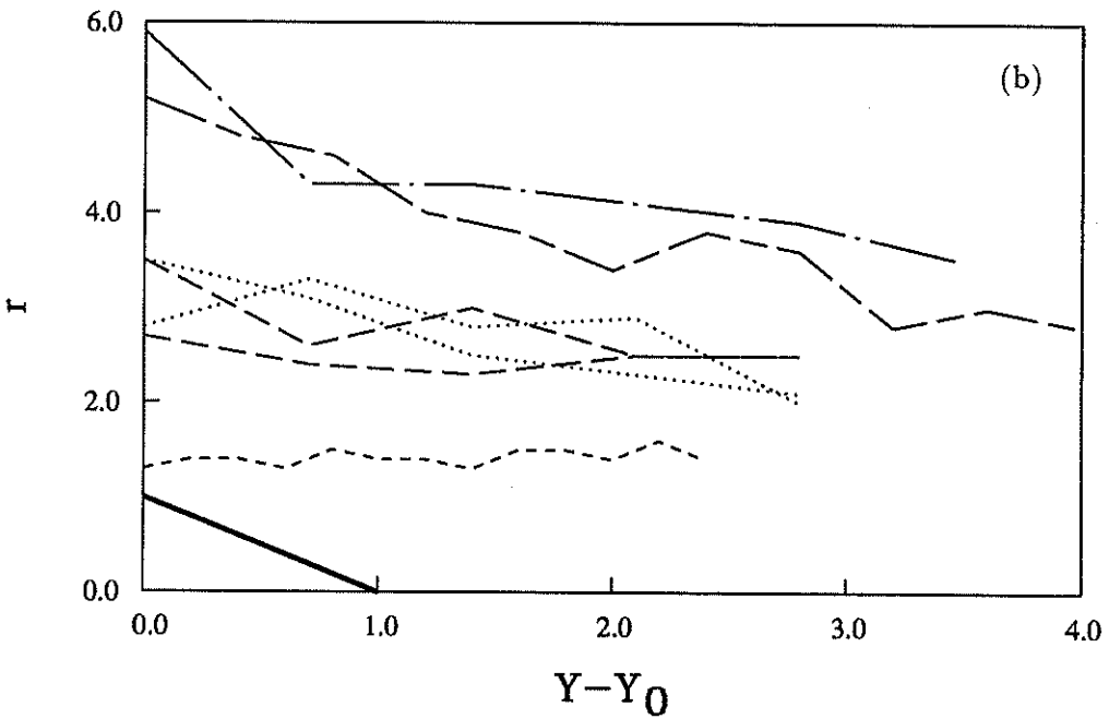
FIGURE 3. Probe separation at extremes of correlations versus relative stationary probe location for X = 27 cm — ; 47 cm - - - ; 57 cm ····· ; 78 cm - · - · ; 88 cm — — — ; 128 cm — · — ; Line with slope equal to -1 ———. (a) Transverse velocity ( v ) in the spanwise ( Z ) direction. (b) Spanwise velocity ( w ) in the transverse ( Y ) direction.
