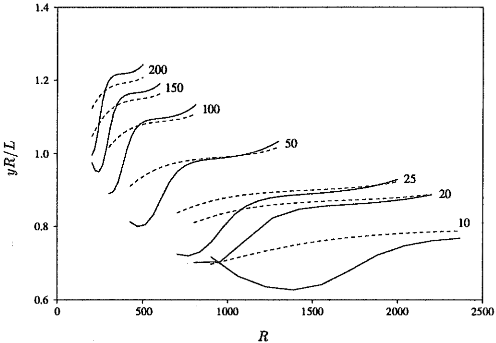
FIGURE 1. Height above wall at which a Blasius boundary layer is most sensitive to direct streamwise forcing, as a function of Reynolds number, for various frequencies f \times 10^6 . Dashed lines define the location of the corresponding critical layer.
