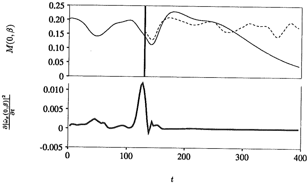
FIGURE 6. Regeneration process of unsustained flow, and modified flow. —, M(0, \beta) ; ----, same flow with \hat{v}, \hat{w}(0, y, n\beta) ( n \neq 0 ) modes multiplied by 1.5 at t = 130.0 (denoted by heavy vertical line); —, \partial|\hat{w}_x(0, y, \beta)|^2/\partial t , due to nonlinear terms only, integrated in y for unmodified flow.
