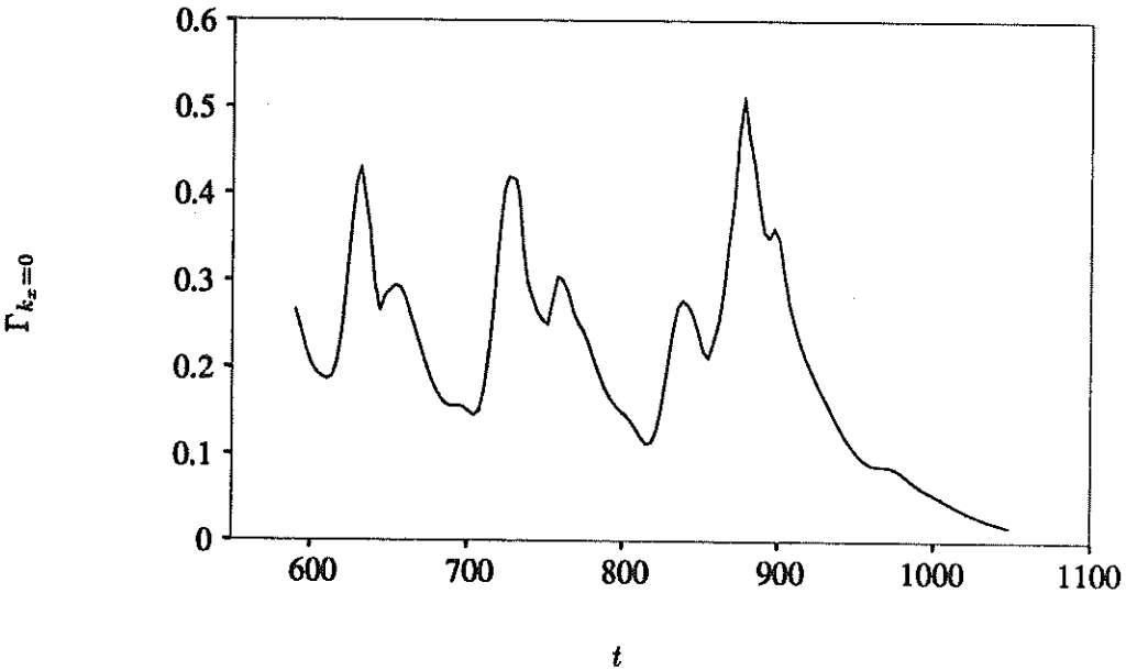
FIGURE 4. Circulation of k_x = 0 modes over last few cycles of flow of Figure 3.
