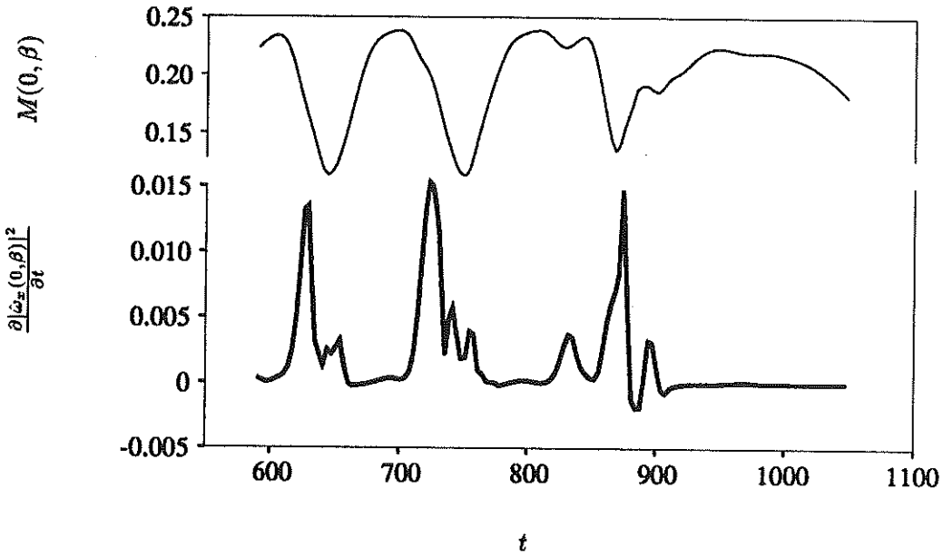
FIGURE 3. Regeneration process over last few cycles of unsustained flow. —, M(0, \beta) ; - - -, \partial|\omega_x(0, y, \beta)|^2/\partial t , due to nonlinear terms only, integrated in y .
