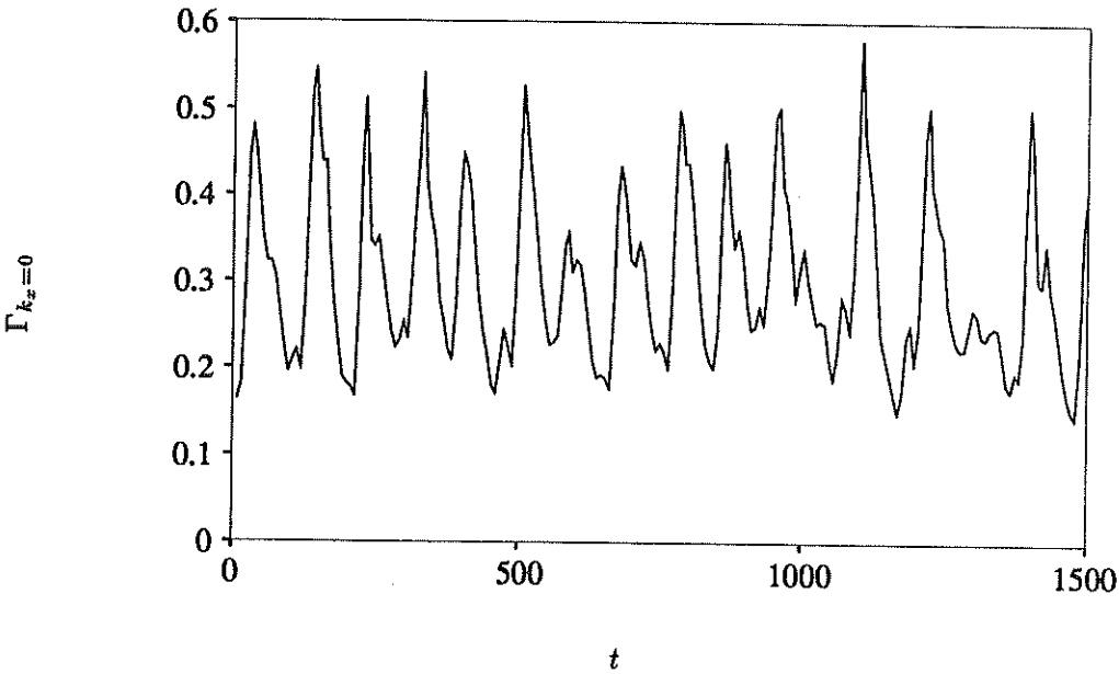
FIGURE 2. Circulation of k_x = 0 modes over many regeneration cycles. Circulation plotted is based on contour that gives the maximum circulation from among all rectangular contours on computational grid points in y - z plane.
