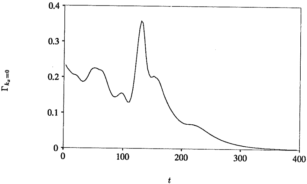
FIGURE 7. Circulation of k_x = 0 modes of unsustained (unmodified) turbulent flow of Figure 6.
