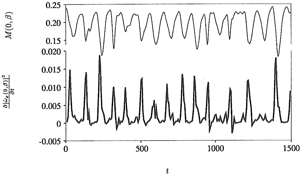
FIGURE 1. Regeneration process over many cycles. —, M(0, \beta) ; —, \frac{\partial |\hat{\omega}_x(0, y, \beta)|^2}{\partial t} , due to nonlinear terms only, integrated in y .
