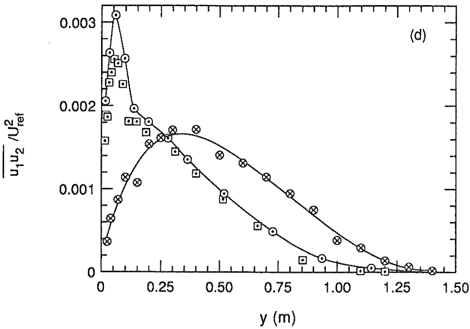
FIGURE 4. Profiles of Reynolds stresses measured in plane and distorted boundary layers: (a) \overline{u_1^2}/U_{ref}^2 , (b) \overline{u_2^2}/U_{ref}^2 , (c) \overline{u_3^2}/U_{ref}^2 , (d) \overline{u_1 u_2}/U_{ref}^2 . For key to symbols see figure 1.
