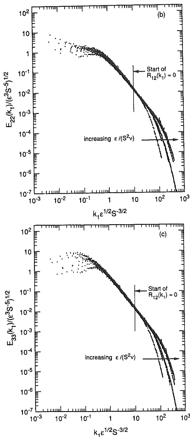
FIGURE 10. Spectra measured at different locations and freestream velocities in the plane and distorted boundary layers non-dimensionalized using \sqrt{\epsilon/S^3} and \sqrt{\epsilon/S} as length and velocity scales respectively. (a) E_{11}(k_1) ; (b) E_{22}(k_1) ; (c) E_{33}(k_1) .
