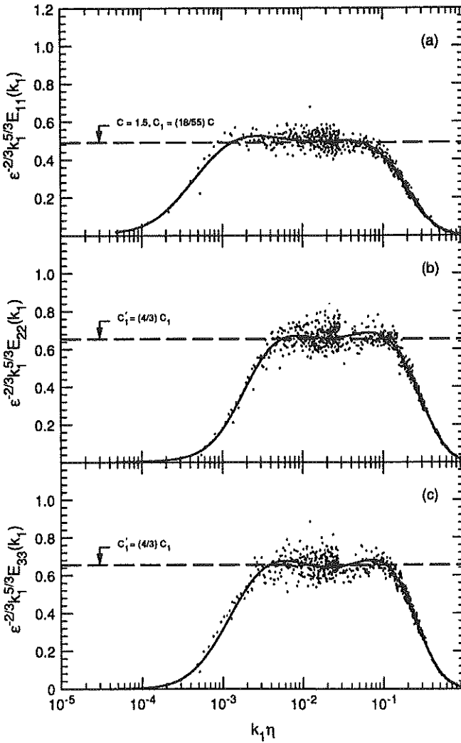
FIGURE 14. Compensated longitudinal and transverse spectra measured at y = 500 mm in the small extra-strain-rate boundary layer at low Reynolds number ( R_\lambda \approx 760 ). Solid lines are the ninth-order, least-square, log-log polynomial fits to the spectral data. (a) u_1 -spectrum; (b) u_2 -spectrum; (c) u_3 -spectrum.
