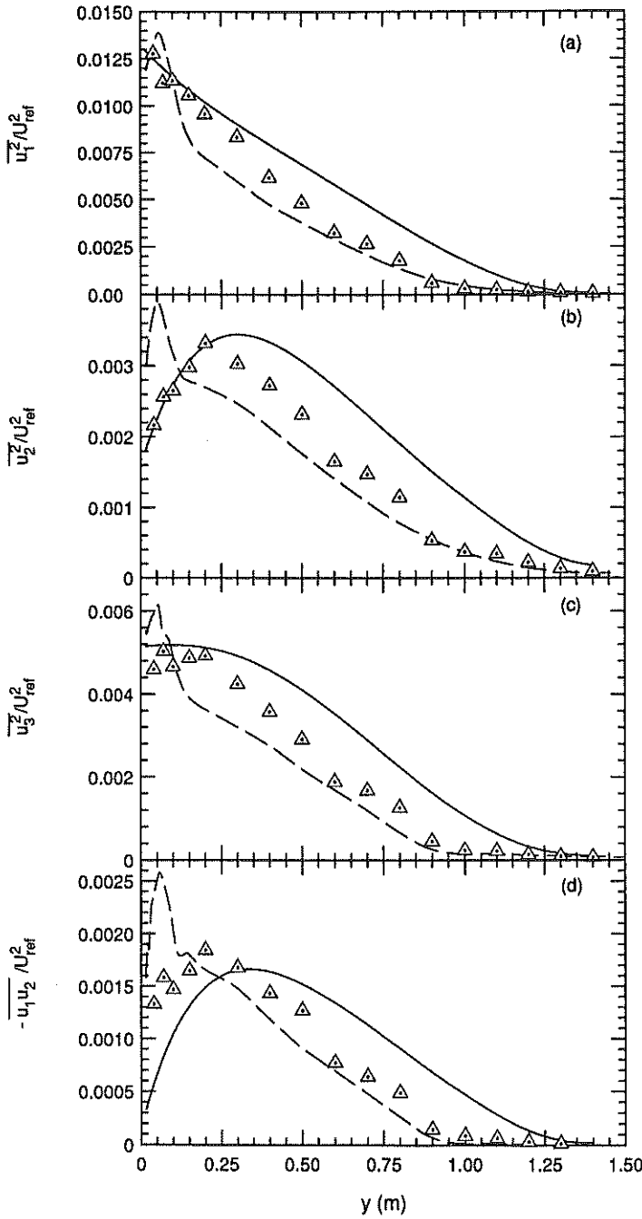
FIGURE 12. Normalized profiles of Reynolds stresses for different boundary layers. (a) \overline{u_1^2}/U_{ref}^2 , (b) \overline{u_2^2}/U_{ref}^2 , (c) \overline{u_3^2}/U_{ref}^2 , (d) -\overline{u_1 u_2}/U_{ref}^2 . For key to symbols see Fig. 11.
