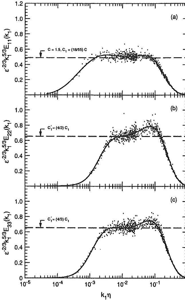
FIGURE 13. Compensated longitudinal and transverse spectra measured at y = 300 mm in the small extra-strain-rate boundary layer at low Reynolds number ( R_\lambda \approx 790 ). Solid lines are the ninth-order, least-square, log-log polynomial fits to the spectral data. (a) u_1 -spectrum; (b) u_2 -spectrum; (c) u_3 -spectrum.
