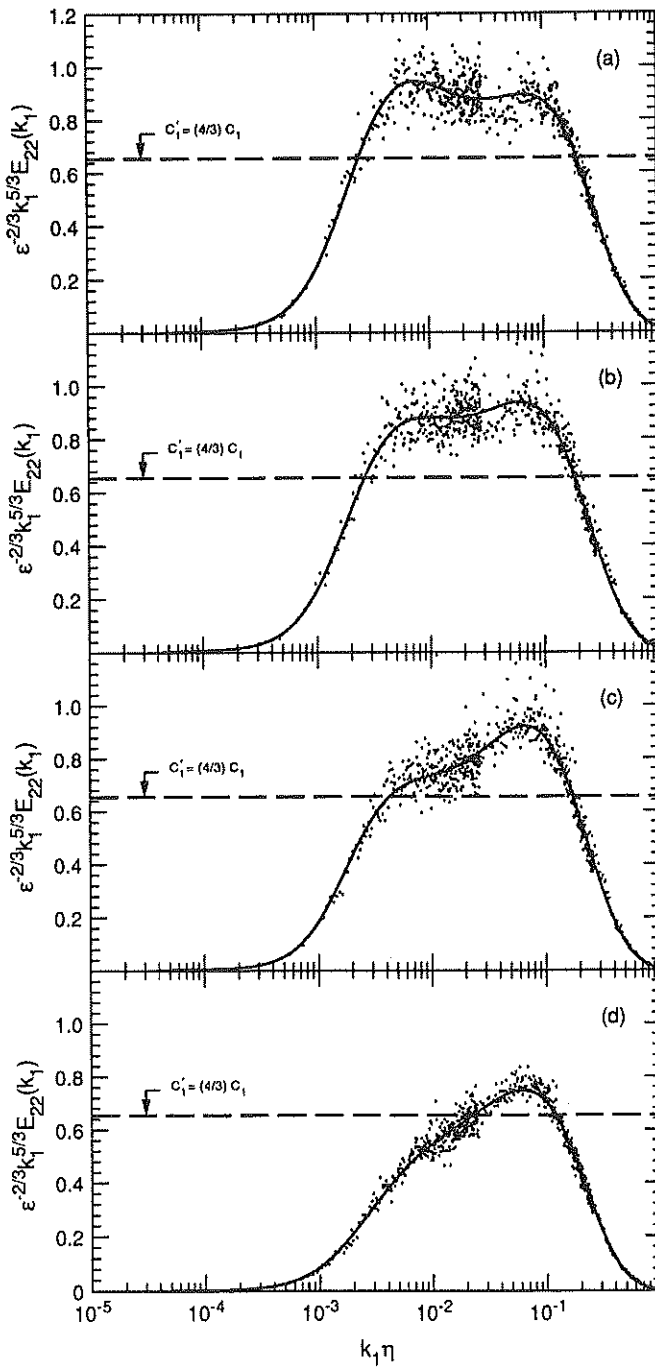
FIGURE 6. Compensated u_2 -spectra measured at different locations in the large extra-strain-rate boundary layer at low Reynolds number. Solid lines are the ninth-order, least-square, log-log polynomial fits to the spectral data. For key to captions for (a)-(d) see Fig. 5.
