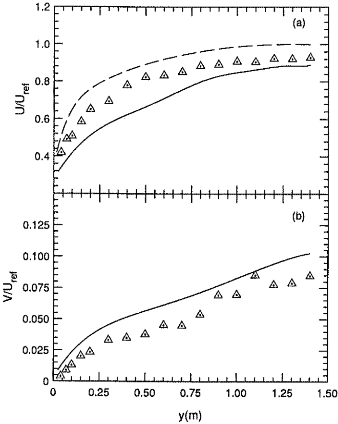
FIGURE 11. Normalized mean-velocity profiles for different boundary layers. (a) U/U_{ref} ; (b) V/U_{ref} . ----, plane boundary layer at low and high Reynolds numbers; —, large extra-strain-rate (with F-18) boundary layer at low and high Reynolds numbers; \Delta , small extra-strain-rate (without F-18) boundary layer at low Reynolds number.
