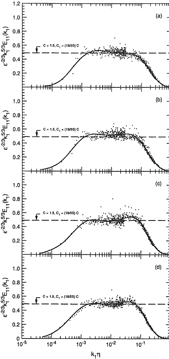
FIGURE 5. Compensated u_1 -spectra measured at different locations in the large extra-strain-rate boundary layer at low Reynolds number. Solid lines are the ninth-order, least-square, log-log polynomial fits to the spectral data. (a) y = 700 mm (outer-layer), R_\lambda \approx 650 ; (b) y = 500 mm (around mid-layer), R_\lambda \approx 820 ; (c) y = 300 mm (maximum shear stress), R_\lambda \approx 800 ; (d) y = 100 mm (inner-layer), R_\lambda \approx 830 .
