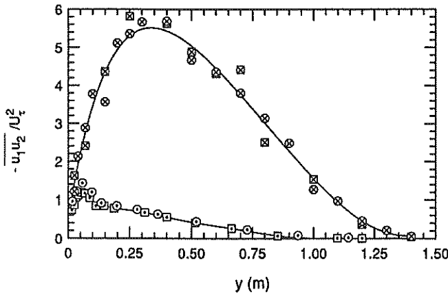
FIGURE 4. Scaling of the Reynolds shear-stress profiles (Fig. 3d) using U_\tau as velocity scale. For key to symbols see Fig. 2.
