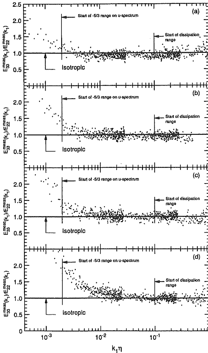
FIGURE 8. Ratios of the measured u_3 -spectra to u_2 -spectra at different locations in the large extra-strain-rate boundary layer at low Reynolds number. For key to captions for (a)-(d) see Fig. 5.
