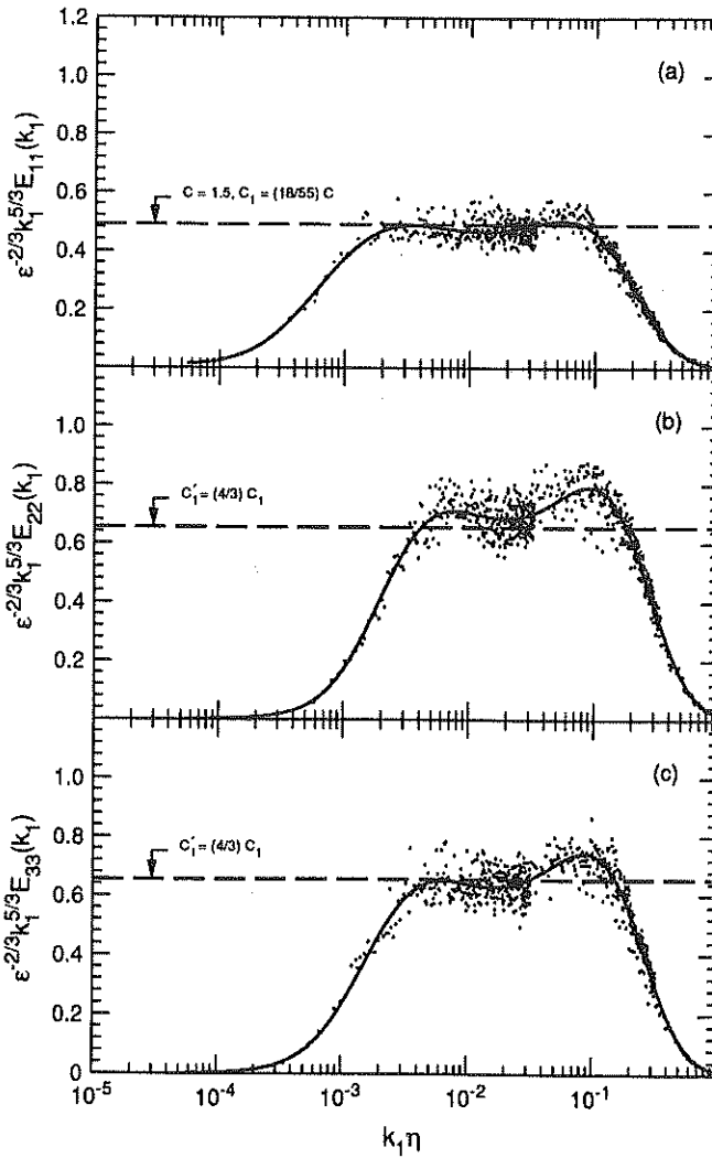
FIGURE 15. Compensated longitudinal and transverse spectra measured at y = 700 mm in the small extra-strain-rate boundary layer at low Reynolds number ( R_\lambda \approx 560 ). Solid lines are the ninth-order, least-square, log-log polynomial fits to the spectral data. (a) u_1 -spectrum; (b) u_2 -spectrum; (c) u_3 -spectrum.
