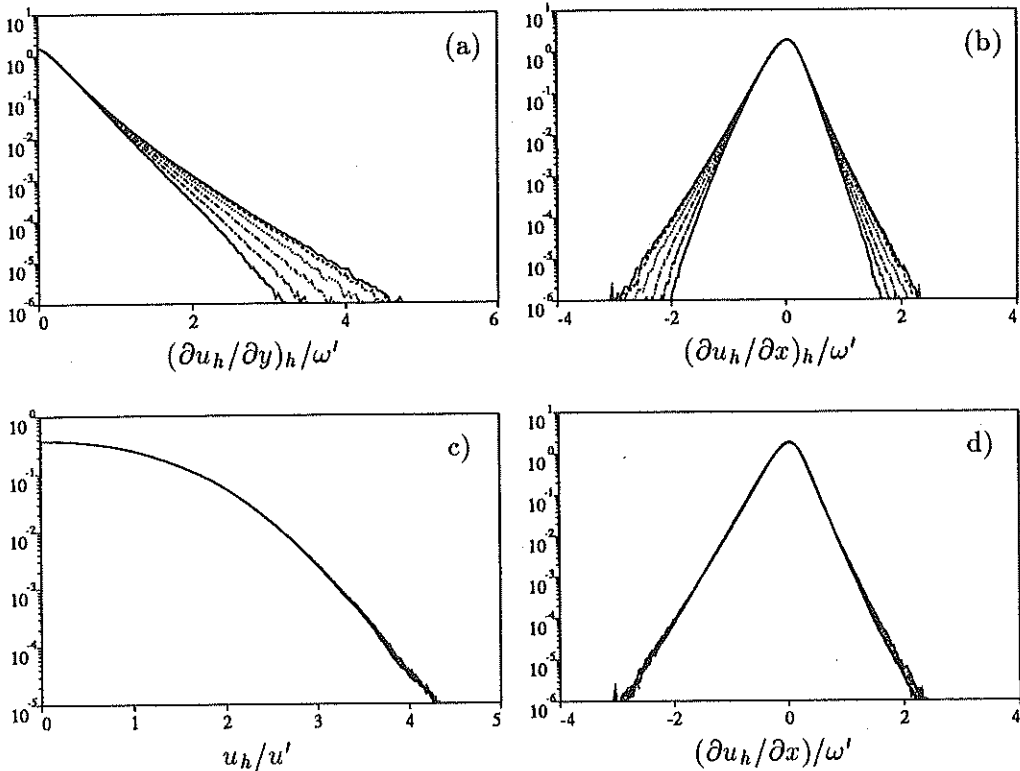
FIGURE 3. Dependence of the probability distributions on experimental resolution. Lines correspond to h/\eta = 0.15, 0.5, 1.5, 3, 5, 7.5 , in order of decreasing intermittency of distributions. Re_\lambda = 92 . (a) Filtered transversal derivatives of filtered velocity. (b) Filtered longitudinal derivatives of filtered velocity. (c) Filtered velocity. (d) True longitudinal derivatives of filtered velocity.
