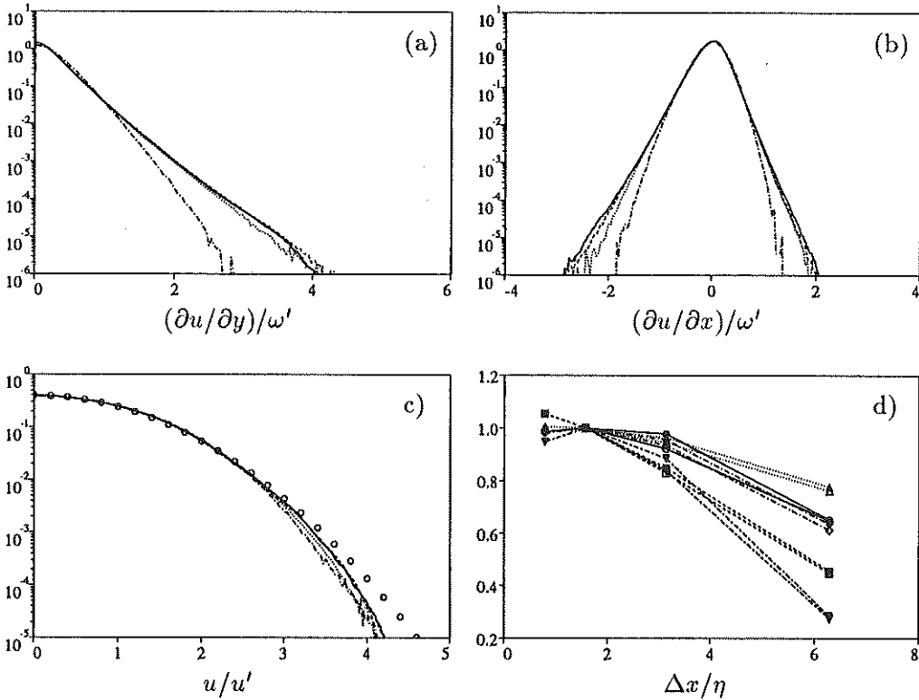
FIGURE 2. Dependence of the probability distributions on numerical resolution. (a-c) Pdf's of velocity and velocity gradients, Re_\lambda = 66 . Lines are as in Fig. 1 and symbols in (c) are the Gaussian distribution. (d) Dependence of the velocity gradient flatness factors on \Delta x / \eta = \pi / k_{\max} \eta . All moments are normalized with their value at k_{\max} \eta = 2 . \circ : F_{3\ell} , \triangle : F_{4\ell} , \square : F_{6\ell} , \diamond : F_{4t} , \nabla : F_{6t} . Solid symbols are Re_\lambda = 66 , open ones, Re_\lambda = 92 .
