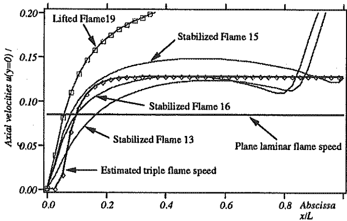
FIGURE 10. Velocity and temperature profiles along wake axis for different stabilized diffusion flames.
