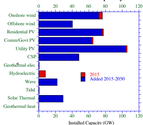
Figure 3. 2015 and proposed 2015-2050 additions of installed capacity of WWS generators for Australia.
