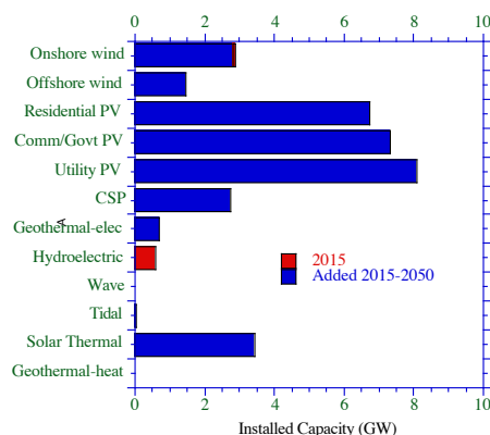
Figure 3. 2015 and proposed 2015-2050 additions of installed capacity of WWS generators for Haiti-Dominican Republic.
