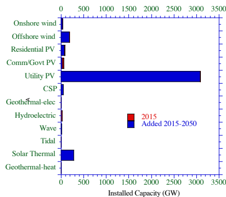
Figure 3. 2015 and proposed 2015-2050 additions of installed capacity of WWS generators for Japan-South Korea.
