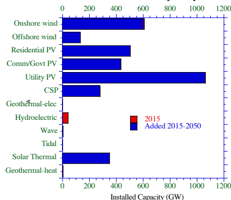
Figure 3. 2015 and proposed 2015-2050 additions of installed capacity of WWS generators for the Mideast.
