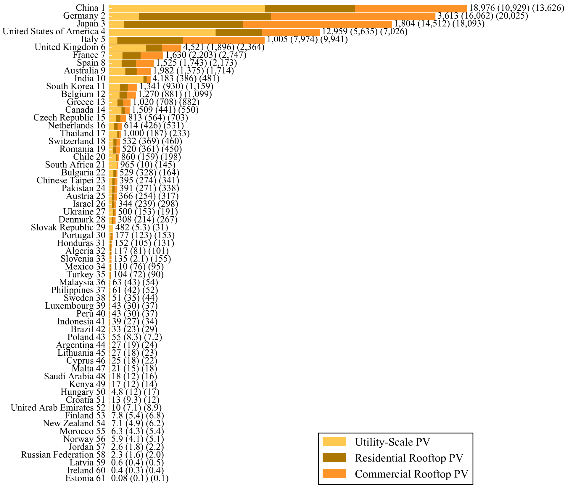
Installed 2015 solar PV capacity (MW) World: 67,334 (util) 70,331 (res) 87,749 (com)
