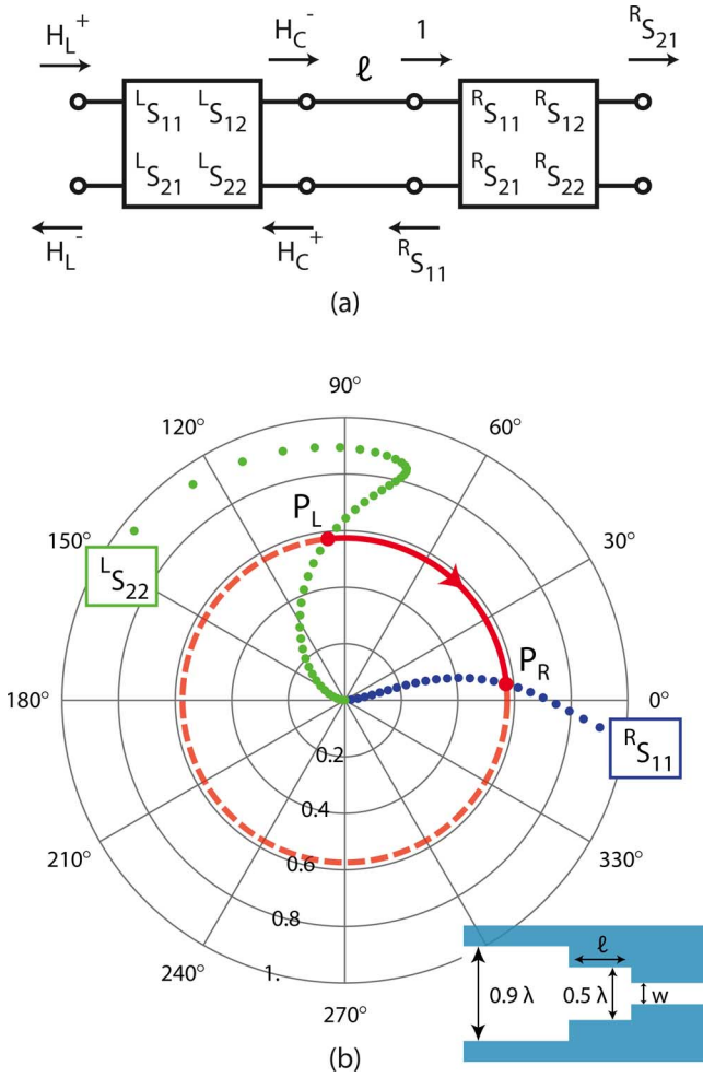
Fig. 4. (a) Schematic diagram of modal propagation. The left and right junctions are shown as boxes with an S matrix description. The center waveguide is shown as a transmission line of length \ell . The source that creates the fields is normalized such that the mode that propagates to the right has a unit magnitude at the input of the right junction. (b) Graphical solution of (11) and (12) on the complex plane. Point P_L is the location of the left junction on the L_{S_{22}} curve where b = 0.9\lambda and b' = 0.5\lambda . Point P_R is the location of the right junction on the R_{S_{11}} curve where b = 0.5\lambda and b' = 0.16\lambda .
