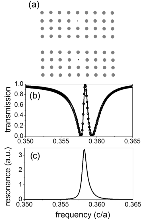
Fig. 5. (a) Schematic of a two-dimensional photonic crystal structure with dielectric rods of radius 0.2a and dielectric constant 11.56. A waveguide is formed by removing one row of dielectric rods. One resonator is formed by reducing the radius of a rod three periods from the waveguide to 0.05a . The second dielectric rod resonator is placed on the opposite side of the waveguide two periods away, by replacing the rod with a rod of radius 0.05a and dielectric constant 12.4. This system is described in terms of a nonorthogonal mode model, since both modes have even symmetry with respect to the mirror plane perpendicular to the waveguide. (b) Transmission spectrum through the waveguide structure. Solid line is the analytic theory and the open circles are FDTD simulations. (c) Resonance amplitudes of the two resonances. Note that the two resonances are not distinguishable since the frequency difference is smaller than the resonance linewidth.
