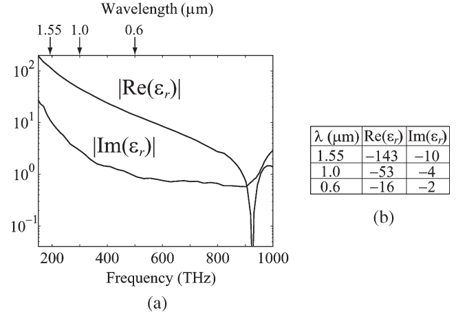
Fig. 2. (a) Absolute values of the real [\text{Re}(\epsilon_r)] and imaginary [\text{Im}(\epsilon_r)] part of the dielectric constant of silver at optical frequencies. \text{Re}(\epsilon_r) < 0 for frequencies below \sim 910 THz. (b) Dielectric constant of silver at selected wavelengths that are considered in this paper.
