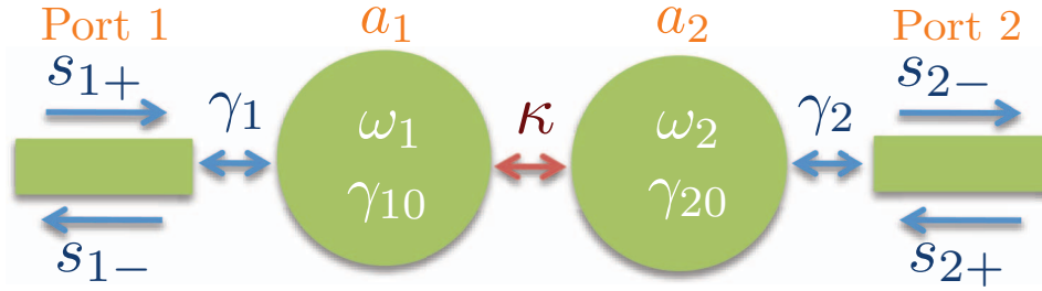
FIG. 1. Coupled mode theory model for the wireless power transfer scheme that utilizes two high-Q resonators. The red arrow represents the wireless power transfer pathway.
