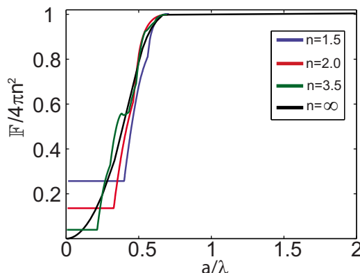
FIG. 3. (Color online) Limit of angular integration of enhancement factor for square lattice.
