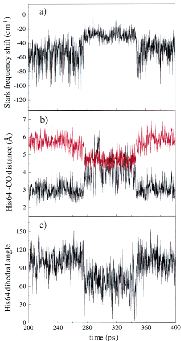
Figure 4. An example of a MD trajectory showing the transition between the R_e state and the B_e state. A transition occurs from R_e to B_e at \sim 280 ps, and then back to the R_e state at \sim 345 ps. (a) The average value of the Stark frequency shift changes abruptly during the transition. (b) The distance between N_e -H (black) and N_\delta of His64 (red) during the trajectory. In the R_e state, N_e -H is much closer to the ligand than N_\delta . In the B_e state, the distances of N_e -H and N_\delta of His64 to the CO are about the same. (c) The dihedral angle of the C_\beta - C_\delta bond changes during the transition from R_e to B_e at \sim 280 ps and then back at \sim 345 ps.
