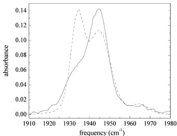
Figure 11. Comparison of the measured IR absorption spectrum (solid line) of the CO stretch in MbCO with that calculated using FFCFs for the N_{\delta} -H tautomer of His64 (dashed line). The linear spectrum for the N_{\delta} -H tautomer is calculated using the same line centers and concentrations used in the calculation of the linear spectrum for the N_{\epsilon} -H tautomer of His64 shown in Figure 9. The agreement between the measured and calculated linear spectrum for the N_{\delta} -H tautomer is quite poor.
