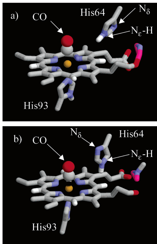
Figure 5. Snapshots of the heme pocket 45 during the MD trajectory shown in Figure 4. (a) The R_e configuration has N_{\epsilon} -H oriented toward the CO, and the N_{\delta} oriented toward the solvent. (b) In the B_e configuration, the imidazole ring of His64 has undergone a rotation around the C_{\beta} - C_{\delta} bond so that N_{\epsilon} -H is oriented away from the CO ligand and N_{\delta} is inside the heme pocket.
