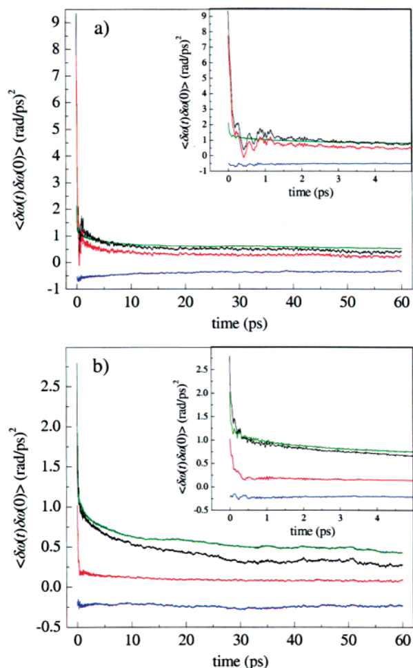
Figure 13. Decomposition of the FFCFs into contributions from His64 and from the rest of the system for the (a) A_3 and (b) A_1 states observed in MD simulations of MbCO. The total contribution (black), contribution from only His64 (red), contributions from all other atoms (green), and the cross-correlations between the His64 and the rest of the system (blue) are all shown. His64 is the dominant dephasing source for the A_3 state. The A_1 state has a substantial portion of the short time dephasing contribution from His64, but the rest of the system contributes appreciably to the dephasing at longer times. The dephasing contribution for His64 is more strongly anticorrelated with its surroundings in the A_3 state.
