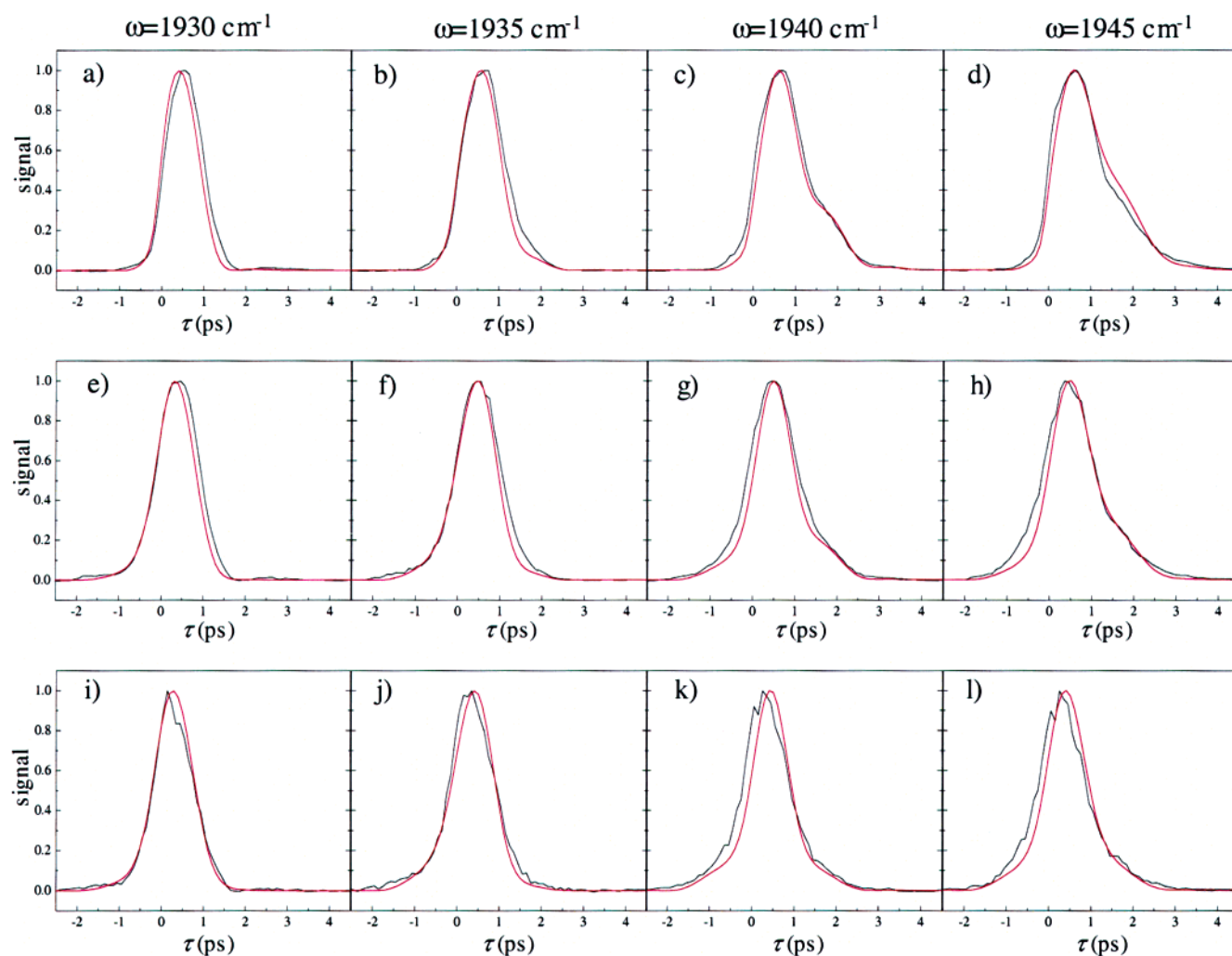
Figure 8. Comparison of the measured vibrational echo data (black) with the calculated vibrational echo data (red) for the N_{\epsilon} -H tautomer of His64. The vibrational echo signals were calculated using the FFCFs shown in Figure 6a. The parameters used in the vibrational echo calculation are listed in Table 2. Spectrally resolved vibrational echo decays are shown for the frequencies 1930, 1935, 1940, and 1945 \text{cm}^{-1} , and T_w = 0 ps (a–d), 2 ps (e–h), and 8 ps (i–l). Vibrational echo decays for a particular frequency as a function of T_w are in columns. The oscillations in the echo decays in panels c and d are due to anharmonic accidental degeneracy beats 38,77,81 between the 0–1 transition of the A_1 line and the 1–2 transition of the A_0 line.
