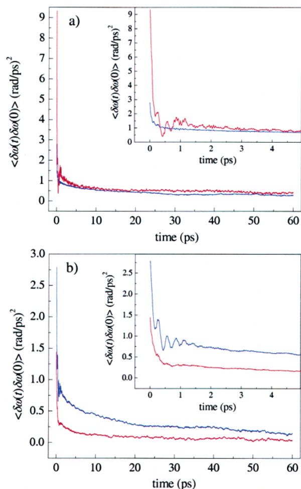
Figure 6. Frequency–frequency correlation functions (FFCFs) for the two tautomers of MbCO derived from MD simulations used to calculate vibrational echo signals. (a) The N_{\epsilon} -H tautomer of His64. The R_e conformer (red) and B_e conformer (blue) both have a fast initial decay over the first few picoseconds, and then continue to decay slowly. The R_e substate has a much larger initial amplitude. The value of the Stark coupling constant \lambda is \lambda = 2.1 \text{cm}^{-1}/(\text{MV}/\text{cm}) . (b) The N_{\delta} -H tautomer of His64. The B_{\delta} conformer (blue) has a larger initial amplitude than the R_{\delta} (red) conformer. The value of \lambda is \lambda = 1.4 \text{cm}^{-1}/(\text{MV}/\text{cm}) .
