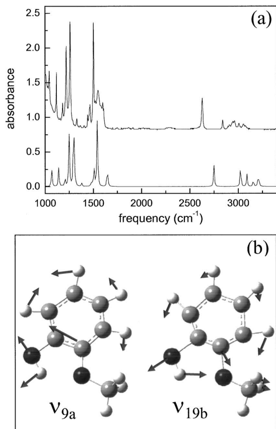
FIG. 8. (a) FTIR spectrum and DFT-calculated spectrum of 2MP. The calculated spectrum is shifted below the experimental spectrum for clarity of presentation. The calculated spectrum is reasonable, but not quantitatively accurate. (b) The nature of the two modes ( \nu_{9a} and \nu_{19b} ) that combine with the first vibrationally excited state of the OD stretch to produce the state |D\rangle that is coupled to |2\rangle the second vibrationally excited state of the OD stretch.
