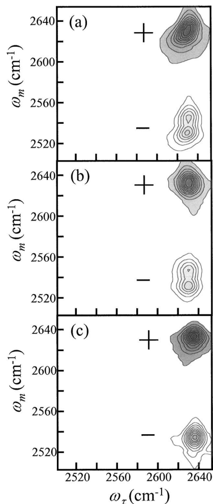
FIG. 3. 2D IR vibrational echo correlation spectra for 2MP and 2MPD4 in \text{CCl}_4 at different T_w 's. (a) 2MP at T_w=200 fs. (b) 2MP at T_w=5 ps. (c) 2MPD4 at T_w=5 ps. Each contour is a 10% change in amplitude. The positive peaks (+) on the diagonal reflect the 0-1 transition, while the negative (-) peaks off-diagonal reflect the 1-2 transition. In (a) and (b) the 1-2 transition displays a doublet, showing that it is not a time-dependent effect. In (c) the 1-2 transition displays a single peak, demonstrating that deuteration of the benzene ring eliminates that doublet.
