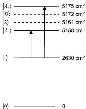
FIG. 6. Energy-level diagram for 2MP in \text{CCl}_4 . The arrows indicate the transition eigenstates (solid lines) that give rise to the doublets in the 1-2 transition regions of the 2D correlation spectra in Figs. 3(a) and 3(b). The dashed lines represent the basis states.
