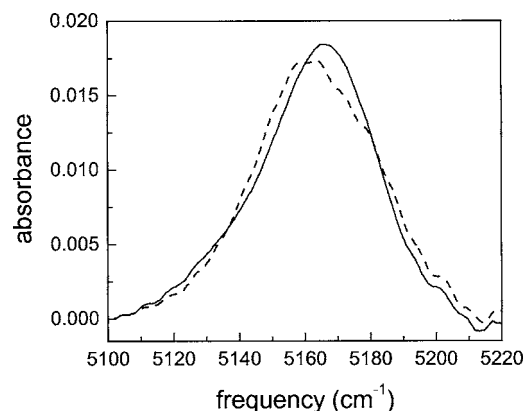
FIG. 7. Near-IR spectra of 2MPD4 (solid curve) and 2MP (dashed curve) in \text{CCl}_4 . The 2MP curve is somewhat broader, but a doublet cannot be resolved.
