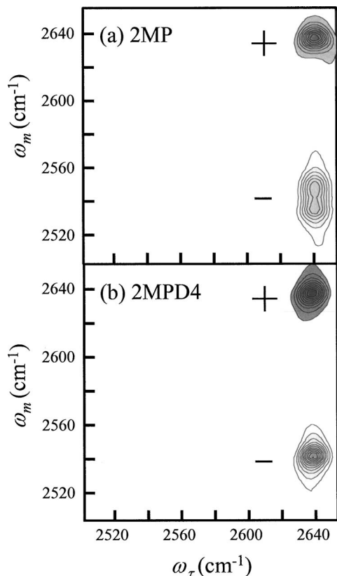
FIG. 4. 2D IR correlation spectra of 2MP (a) and 2MPD4 (b) in hexane, which demonstrate that the appearance of a doublet or a singlet does not depend on the specific solvent as the spectra are basically the same as those in Fig. 3 for which the data were taken in \text{CCl}_4 .
