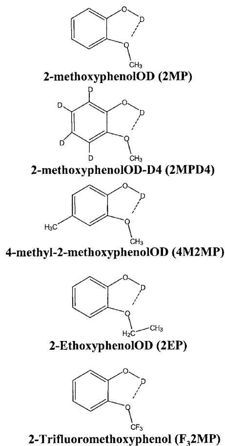
FIG. 1. Structures, names, and abbreviations for the five phenol-OD (hydroxyl H replaced by D) derivatives used in the experiments.
