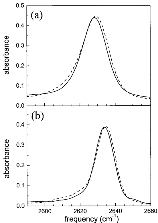
FIG. 2. FTIR spectra of OD Stretch of 2MP and 2MPD4 in (a) \text{CCl}_4 and (b) hexane.
