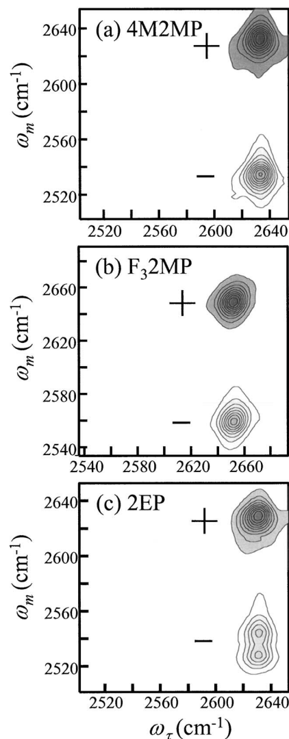
FIG. 5. 2D IR correlation spectra of 4M2MP (a), \text{F}_3\text{2MP} (b), and 2EP (c) in \text{CCl}_4 . The presence of the doublet in the 1-2 transition is influenced by chemical substitution.
