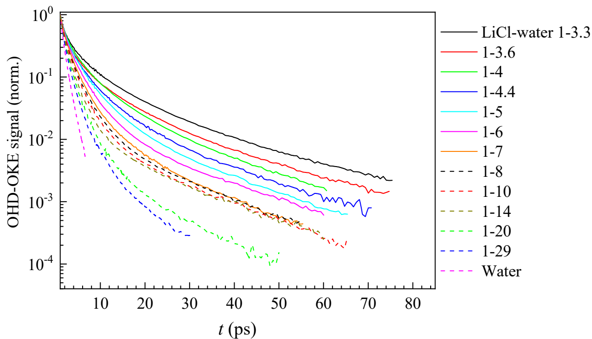
Figure S1: OHD-OKE decays of water and concentration aqueous LiCl solutions. See legend for LiCl-water ratios. Decays were normalized at 1 ps. The decays slowed down with increasing LiCl concentration.
