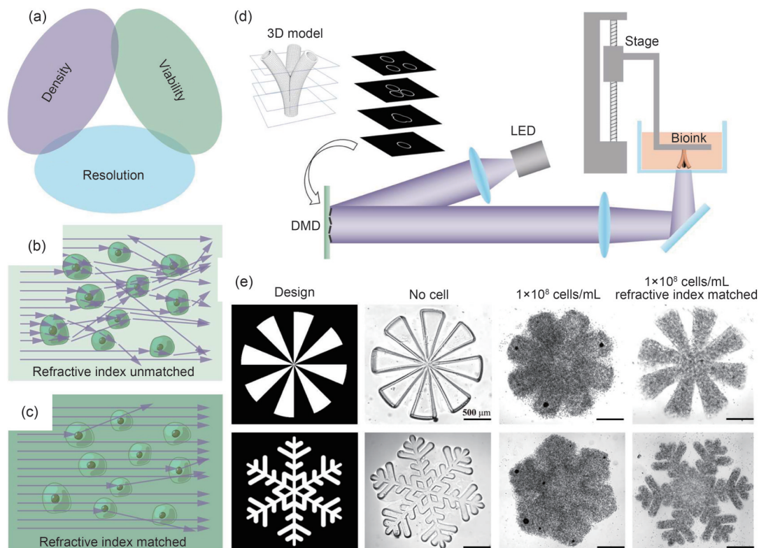
Fig. 7 Achieving high fabrication resolution in high-cell-density bioinks. (a) The “impossible trinity” in bioprinting: high cell density, high cell viability, and high fabrication resolution. Schematics showing light propagation in refractive-index-unmatched (b) and refractive-index-matched (c) bioinks, showing reduced light scattering in the matched system. (d) Working principle of the DLP-based bioprinter. (e) Printing resolution comparison among three different bioink compositions: bioink without cells, bioink with 1 \times 10^8 cells/mL, and refractive-index-matched bioink with 1 \times 10^8 cells/mL (scale bars: 500 \mu\text{m} ). Reproduced from [121], licensed under CC BY 4.0
