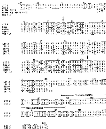
Fig. 5. Lyt-2 homology to other immunologically relevant proteins. Using the BIONET programs IFIND and ALIGN and the protein homology search program of Lipman and Pearson (29), the deduced Lyt-2 protein sequence was aligned against Leu-2 and the most significantly homologous V region sequence of mouse \kappa light chain, human heavy chain Ig, and the V-like region of Thy-1.1. Homologies of these proteins to Lyt-2 are boxed. The cysteines proposed to make the intrachain disulfide bond to form an Ig-like domain in Lyt-2 and Leu-2 are marked by arrows. The transmembrane region of Lyt-2 is indicated. Amino acids are identified by the single letter code.
