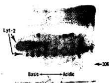
FIG. 3. Two-dimensional gel electrophoresis of the Lyt-2 molecule. A detergent lysate from surface 125 I-labeled transfectants generated by using p6CCA DNA was immunoprecipitated with anti-Lyt-2 antibody (53-6.7). The first dimension was a charge separation with the acidic side on the right and the basic side on the left. The second dimension was NaDodSO 4 /10% polyacrylamide slab gels from the top to the bottom under reducing conditions. 30K, 30 kDa.
