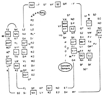
Fig. 6. The Lyt-2 sequence (bold lettering) was mapped, by homology to the human Ni heavy chain V region sequence (italic lettering), onto a two-dimensional representation of the \beta -pleated sheet structure of the Ig heavy chain V region domain (39). Numbering is from NH 2 -terminal of Lyt-2 sequence. Boxed residues indicate homology. Asterisks mark invariant heavy chain Ig V region residues. Shaded regions cover the hypervariable region of heavy chain Ig V domain.
