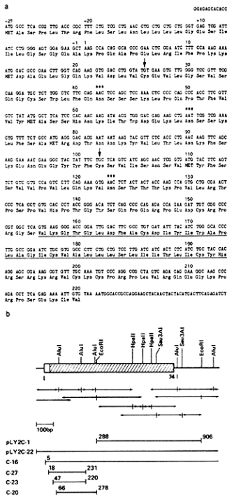
FIG. 2. (a) Nucleotide and amino acid sequence derived from thymocyte cDNA clones encoding Lyt-2. Transmembrane region is underlined. Cysteine residues believed to participate in intrachain disulfide bonding are marked by arrows. Possible N-linked glycosylation sites are marked by asterisks. The 27 amino acid leader peptide is marked as -27 to -1 . Mature peptide is marked from 1 to 220. (b) Restriction endonuclease maps of Lyt-2 cDNA clones. Protein coding region is boxed. Shaded region is mature protein after cleavage of leader peptide. DNA sequence strategy is presented below the map. Numbering refers to nucleotide sequence within each clone relative to the ATG of NH_2 -terminal methionine.
