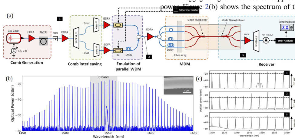
Fig. 2. (a) Experimental setup for WDM-MDM microcomb data transmission. DC Var, variable DC voltage; EDFA, erbium-doped fiber amplifier; FBG, fiber Bragg grating; IM, intensity modulator; PhCR, photonic crystal ring resonator; PIN-TIA-LA, PIN photodiode transimpedance amplifier and limiting amplifier. (b) Optical spectrum of 400 GHz FSR PhCR comb with C-band highlighted (inset: scanning electron micrograph of sinusoidal nanopattern on inner edge of ring). (c) Optical spectrum of PhCR comb pulse in C-band range at various points in the setup; 1, 2, 3 as highlighted in (a). Spectrum 3 is taken for MDM CH 3.
