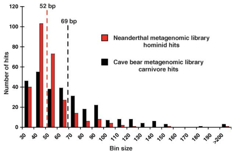
Fig. 2. Size distribution, plotted in 10-bp bins, of Neanderthal and cave bear sequences obtained from metagenomic libraries by Sanger sequencing of individual clones. The average hit size in each case is indicated by a dotted line.
