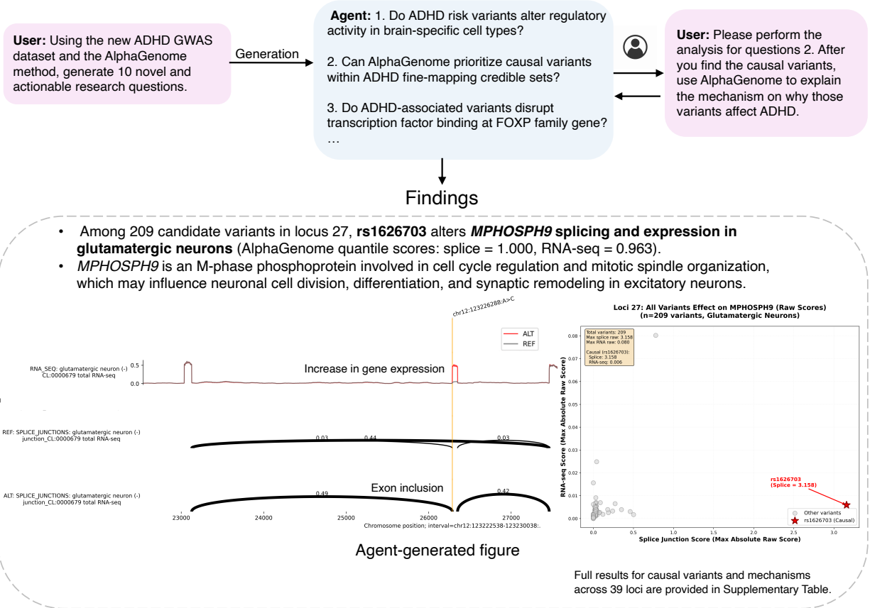
Figure 5: Paper2Agent enables autonomous AI-driven collaboration and genomic discovery. (A) Paper2Agent transforms scientific papers into Model Context Protocol (MCP) resources for both methods and data, allowing AI co-scientist to integrate them and autonomously generate novel hypotheses and actionable research plans. (B) Using the ADHD GWAS dataset and the AlphaGenome method MCPs, the agent autonomously generates and tests scientific hypotheses, identifies causal variants, and interprets molecular mechanisms. The agent identified rs1626703 as a likely causal variant among 209 candidate variants. The agent then showed computationally using AlphaGenome that rs1626703 alters splicing of MPHOSPH9 and increases its expression in glutamatergic neurons, revealing a plausible causal mechanism for ADHD risk.
