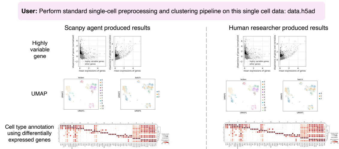
Figure 4: Overview of the Paper2Agent-generated Scanpy agent. (A) Construction of the Scanpy MCP server and agent. (B) MCP prompts encode a standardized single-cell preprocessing and clustering pipeline. (C) Agent reproduces human researcher results, requiring only the dataset path as input.
