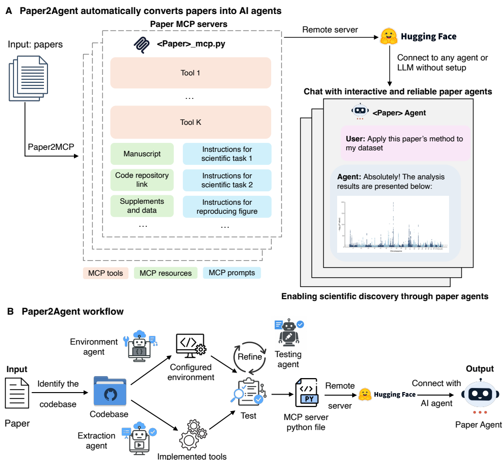
Figure 1: Overview of the Paper2Agent. (A) Paper2Agent turns research papers into interactive AI agents by building remote MCP servers with tools, resources, and prompts. Connecting an AI agent to the server creates a paper-specific agent for diverse tasks. (B) Workflow of Paper2Agent. It starts with codebase extraction and automated environment setup for reproducibility. Core analytical features are wrapped as MCP tools, then validated through iterative testing. The resulting MCP server is deployed remotely and integrated with an AI agent, enabling natural-language interaction with the paper’s methods and analyses.
