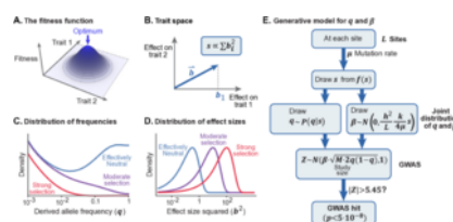
Fig 1. The model.
