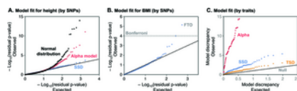
Fig 4. Model fit.
