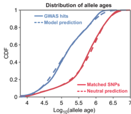
Fig 5. Allele ages.
