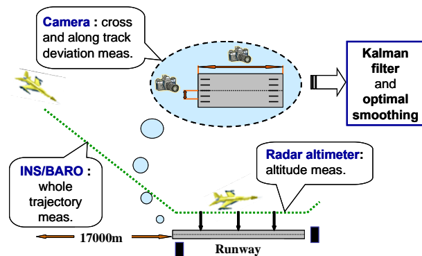
Fig. 2. Position estimation procedure in AFIS
