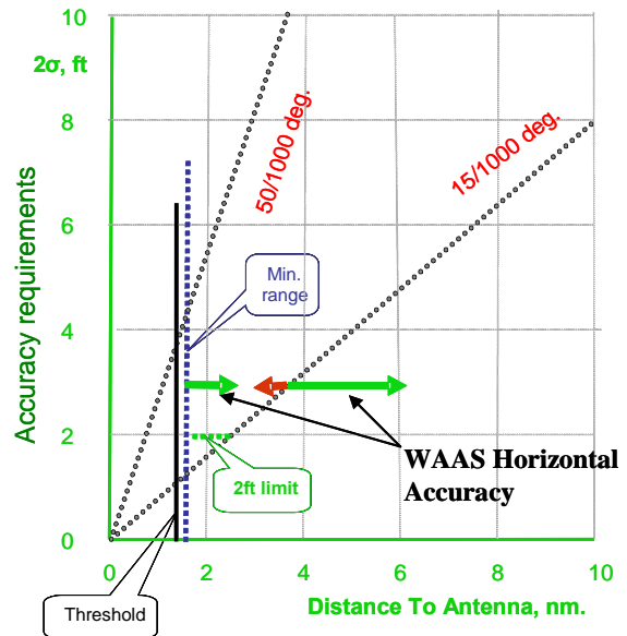
Fig. 4. Comparison of WAAS accuracy and ILS calibration accuracy requirements in horizontal
