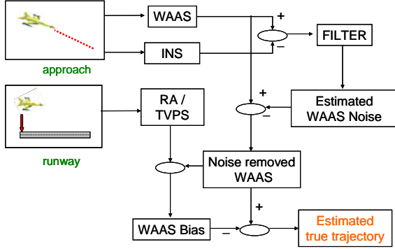
Fig. 8. Algorithm of WAAS-Aided FITS
