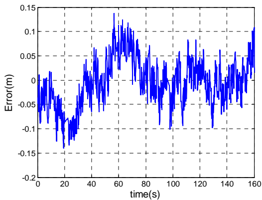
Fig. 14. The residual errors of the estimated WAAS noise
