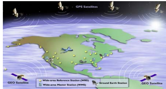
Fig. 1. Wide Area Augmentation System (courtesy of FAA)
