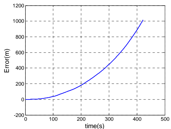
Fig. 17. Simulated horizontal error for a tactical grade
