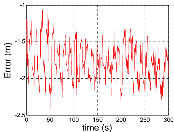
Fig. 5. WAAS airborne position error
