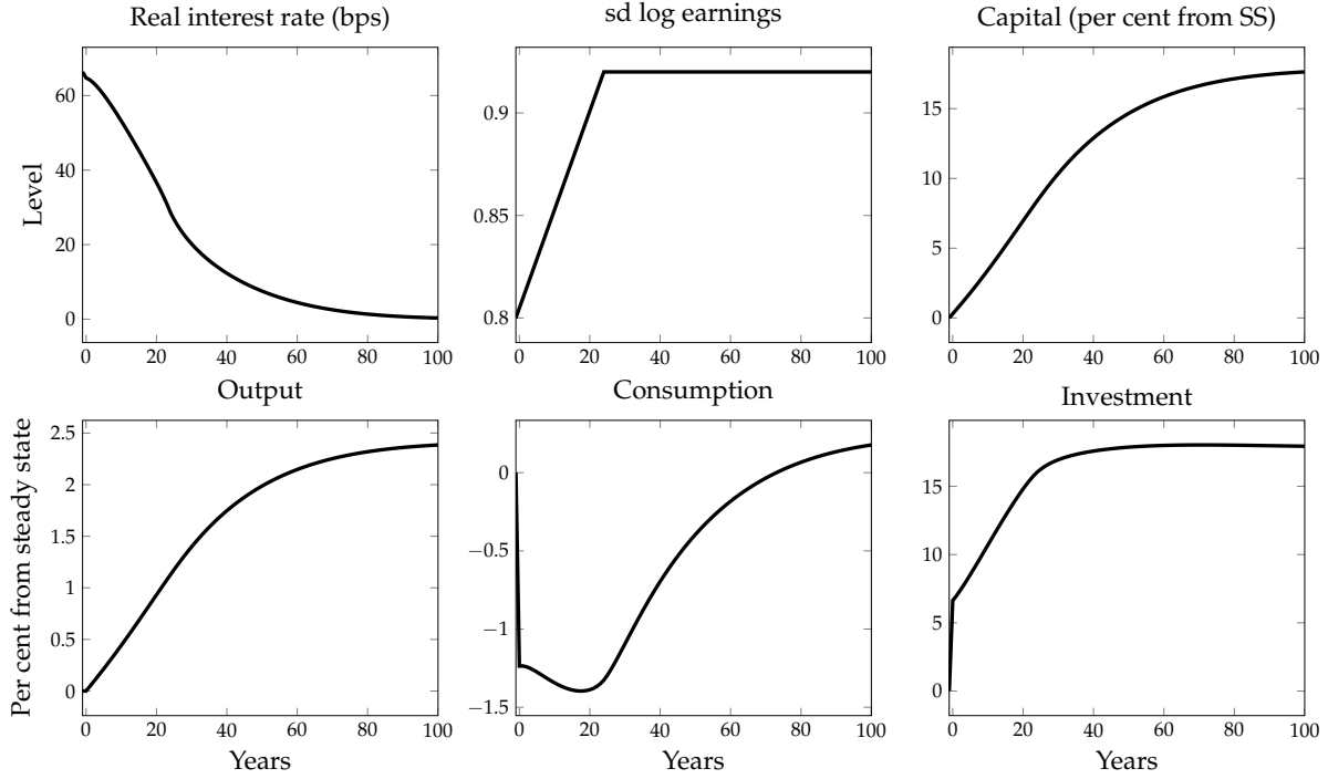
Figure 9: Inequality and the r^* decline
