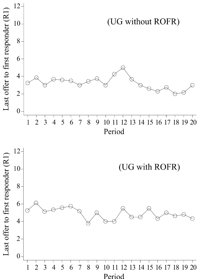
Fig. 6. First responders' average rejected offer ( RI ) before proposer made a new offer to the second responder in the traditional UG.
