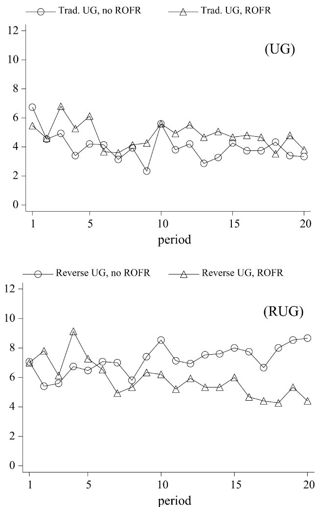
Fig. 2. Average payoffs of the first responder over time (including disagreements), in the traditional UG (UG) and the reverse UG (RUG).
