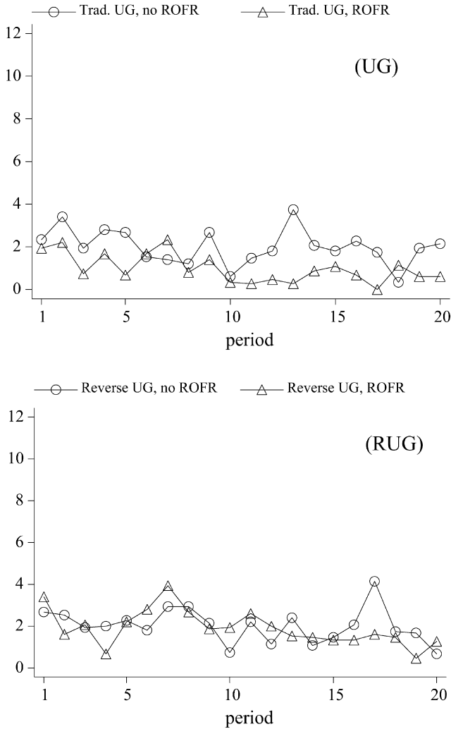
Fig. 3. Average payoffs of the second responder over time, (including disagreements) in the traditional UG (UG) and the reverse UG (RUG).
