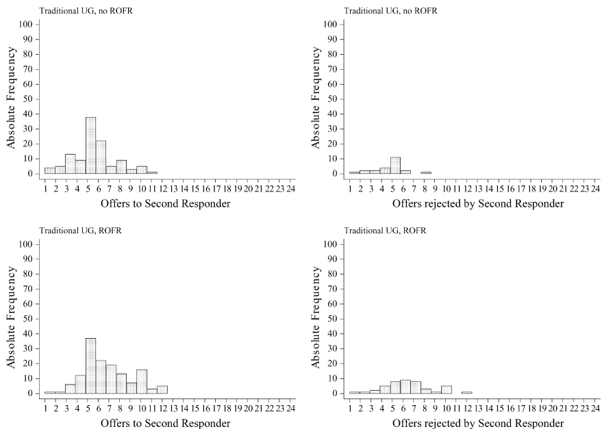
Fig. 10. Offers made to the second responder (left) and offers rejected (right) in the Traditional UG without (top) and with (bottom) ROFR.
