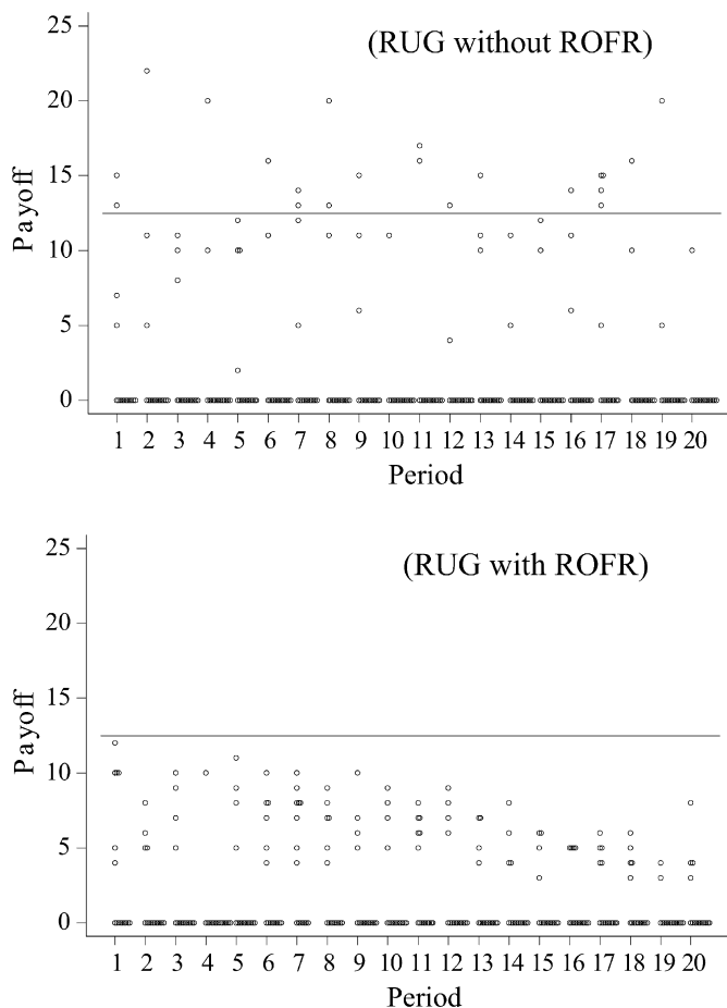
Fig. 4. Dotplots of payoffs of second responders in the reverse UG.
