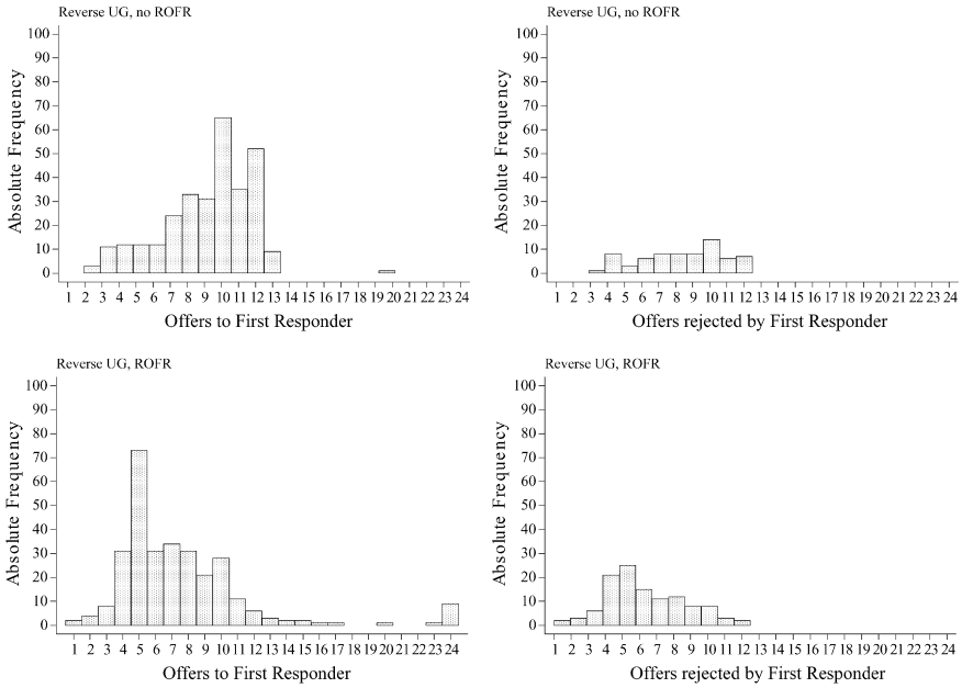
Fig. 11. Offers made to the first responder (left) and offers rejected (right) in the Reverse UG without (top) and with (bottom) ROFR.
