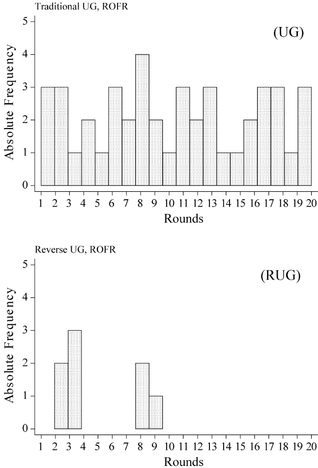
Fig. 8. Histogram of disagreements in the UGs with ROFR over time.
