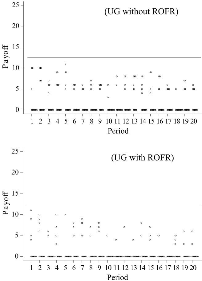
Fig. 5. Dotplots of payoffs of second responders in the traditional UG.
