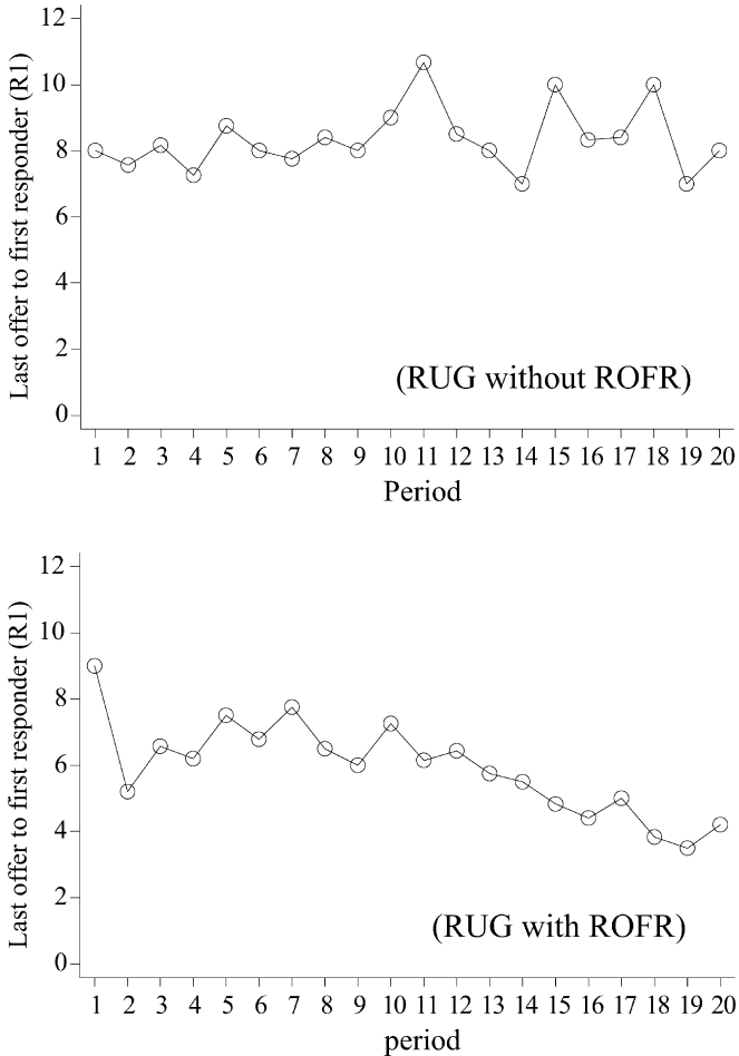
Fig. 7. First responders’ average last rejected offer ( R1 ) before proposer decided to switch to second responder in the reverse UG.
