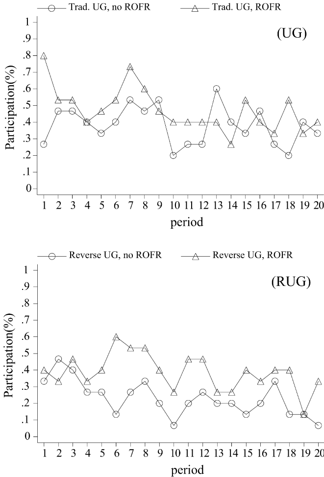
Fig. 13. Observed frequency of participation of the second responder over time.
