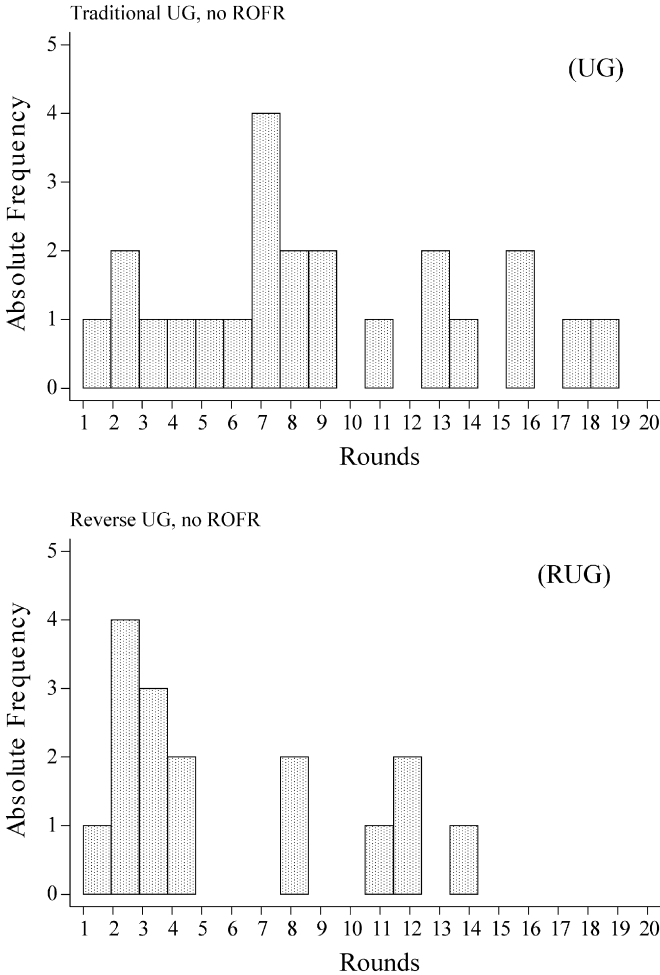
Fig. 14. Histogram of disagreements for the UGs without ROFR over time.
