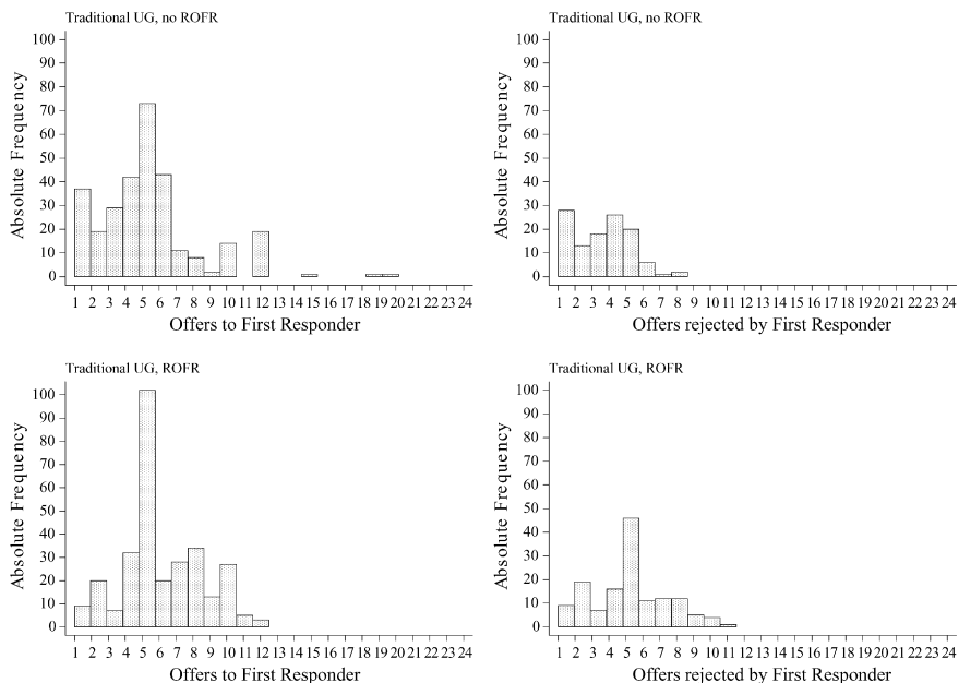
Fig. 9. Offers made to the first responder (left) and offers rejected (right) in the Traditional UG without (top) and with (bottom) ROFR.
