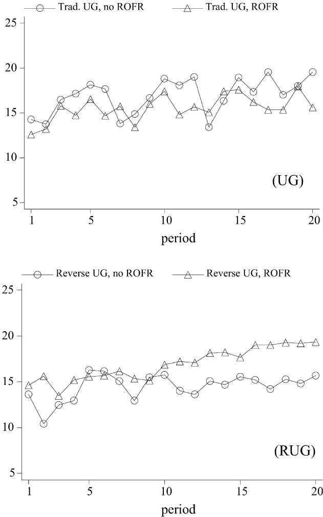
Fig. 1. Average payoff of proposers over time (including disagreements), with and without the ROFR, in the traditional ultimatum game (UG), and the reverse ultimatum game (RUG).
