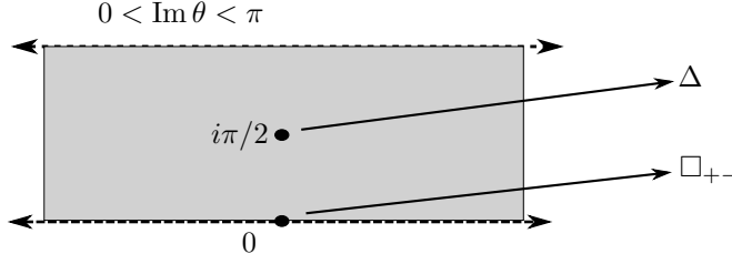
FIGURE 4. The index of L_\theta is constant in the grey region by the standard continuity of the index for Fredholm families. In Theorem 4.3 we show the continuity of the index extends up to the dashed line at bottom, i.e. to L_{+-} .
