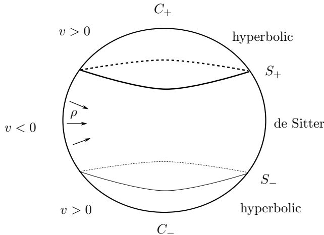
FIGURE 1. \rho equals zero exactly on the boundary and has non-vanishing differential there.
