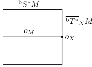
FIGURE 2. The radially compactified cotangent bundle \overline{bT^*M} near \overline{bT^*}_X M ; the cosphere bundle {}^bS^*M , viewed as the boundary at fiber infinity of \overline{bT^*M} , is also shown, as well as the zero section o_M \subset \overline{bT^*M} and the zero section over the boundary o_X \subset \overline{bT^*}_X M .
