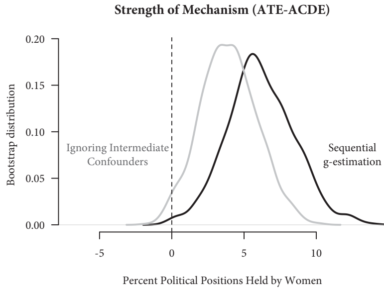
FIGURE 7. Bootstrap Distributions of the Difference Between the ATE and ACDE
