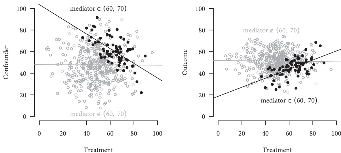
FIGURE 2. Simulated Data Showing the Problem with Conditioning on a Posttreatment Variable
