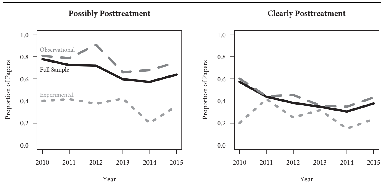
FIGURE 1. Proportion of Papers Implicitly or Explicitly Estimating Causal Relationships that include a Posttreatment Variable
