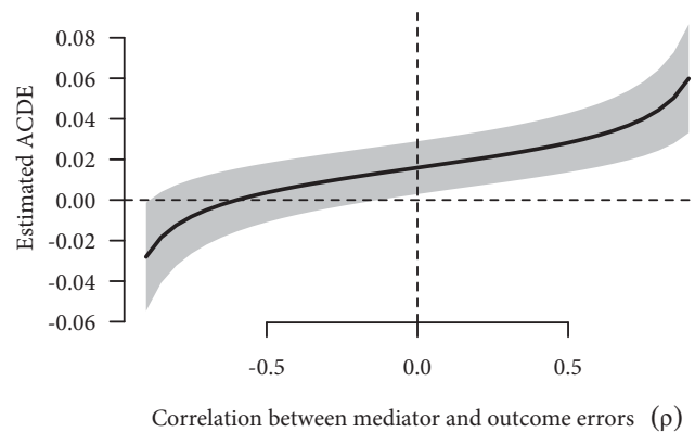
FIGURE 6. Sensitivity Analysis for Fearon and Laitin (2003)
