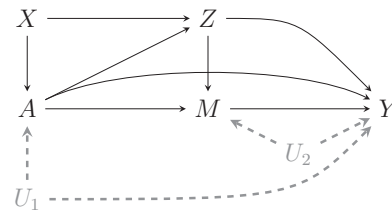
FIGURE 4. Directed Acyclic Graph Showing a Violation of Sequential Unconfoundedness
