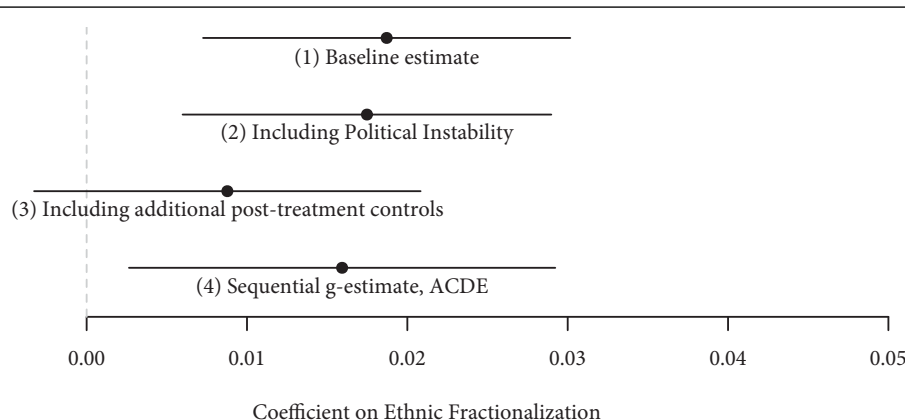
FIGURE 5. Estimated Effects of Ethnic Fractionalization on Civil War Onset
