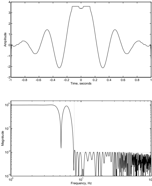
Fig. 2. The impulse response and frequency response of the optimal filter.
