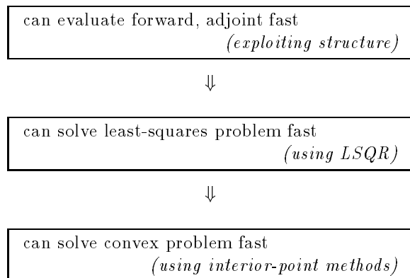
Fig. 1. Exploiting problem structure to efficiently solve convex problems.
