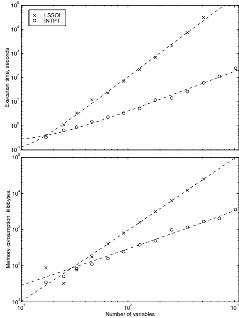
Fig. 3. Execution times and memory consumption for the filter design example.
