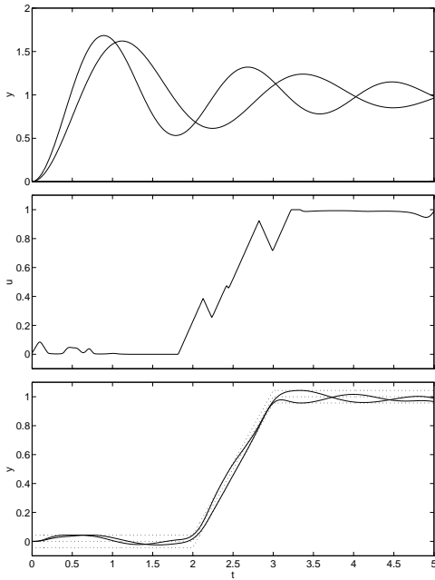
Fig. 4. Step responses, control input, and output trajectories, respectively, for the robust input design example.
