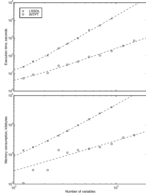
Fig. 8. Execution times and memory consumption for the MIMO input design example.
