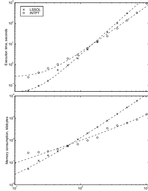
Fig. 5. Execution times and memory consumption for the robust input design example.
