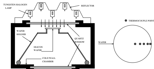
Fig. 6. An experimental rapid thermal processing (RTP) configuration.
