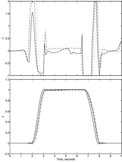
Fig. 7. Control inputs and output trajectories of the MIMO control design example.
