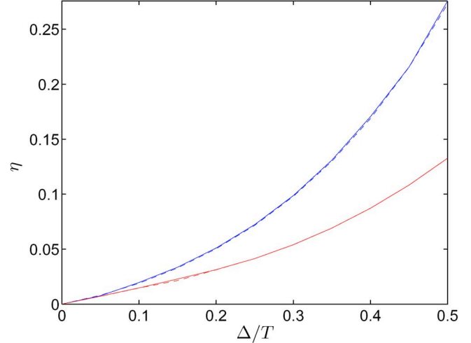
Fig. 1. Top two curves. Lower (dashed) and upper (solid) bounds on \eta with K = K_{lqr} . Bottom two curves. Lower (dashed) and upper (solid) bounds on \eta , for K = K^* , synthesized to minimize the bound on \eta (for each value of \Delta ).
