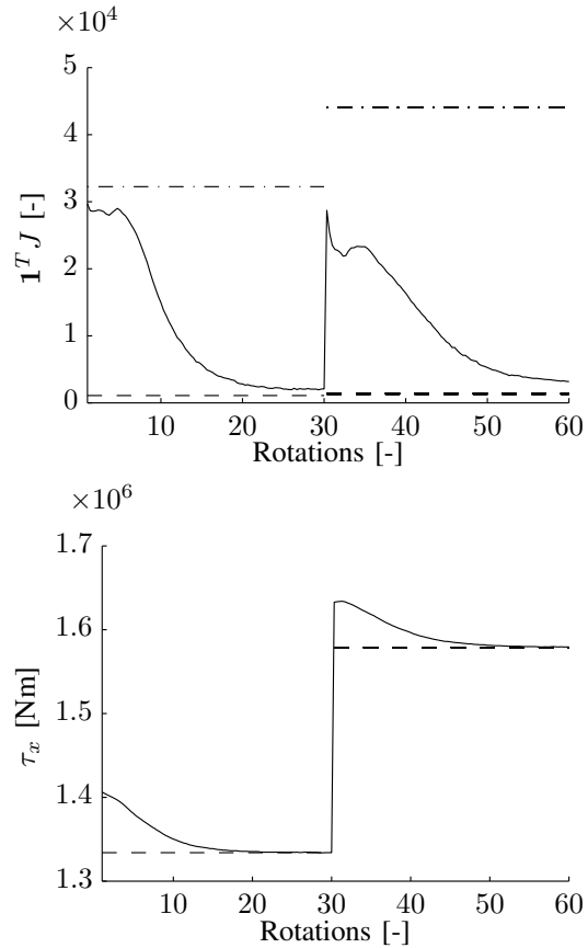
Fig. 8. (Top) The AC-load 1^T J evaluated after each full rotation (solid) compared to the response of using constant pitch profile (dotted dash) and using the optimized pitch profile p^{t.o.}(\theta) (dashed). (Bottom) The output torque \tau_x (solid), along with the set-points (dashed).
