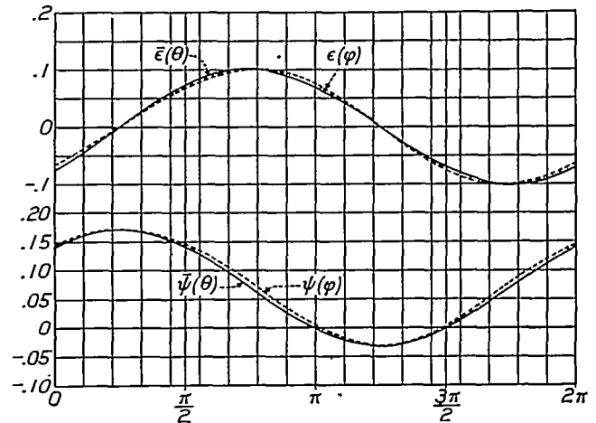
FIGURE 25.—The \bar{\psi}(\theta) and \bar{\epsilon}(\theta) curves for the airfoil in Figure 24
