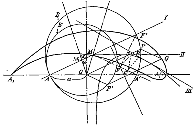
FIGURE 22.—The Joukowsky airfoil
