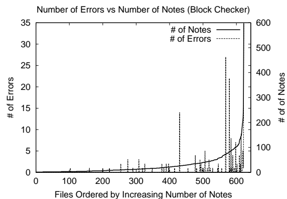
Figure 13: A view of the Block errors found in the entire Linux 2.4.1 kernel. Files are numbered by the number of notes and placed in sorted order on the x-axis. For random coin tosses one would expect the number of errors to be a relatively stable fraction of the number of notes. The absolute number of notes in each file is plotted on the right y-axis, while the absolute number of errors in each file is plotted on the left y-axis.
