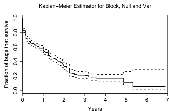
Figure 11: A Kaplan-Meier survival curve that shows the probability of a bug living longer than a given number of years. The dotted curves show the 95% confidence band. This estimator was computed using only bugs from low false positive checkers (Block, Null, and Var).
