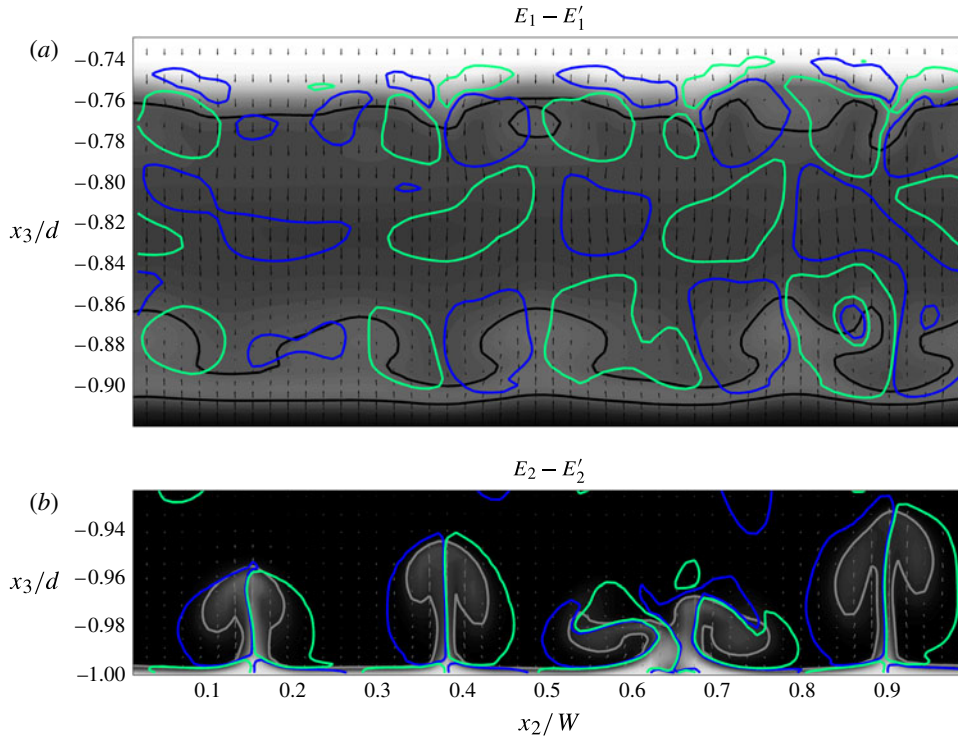
FIGURE 9. An x_2 - x_3 slice through the billow (a) and nose of the upslope surge (b) in figure 6(e). Slice locations are shown in figure 13(e) by sections E_1 - E'_1 and E_2 - E'_2 , respectively. Shading represents the density field using the same color scale as figure 2. Arrows represent velocity vectors ( u_2, u_3 ). Bold contour lines represent \rho/\rho_0 = 1.005 in (a) and \rho/\rho_0 = 1.011 in (b) and depict cross-stream plumes developing due to unstable stratification. Streamwise vorticity is shown by blue ( \omega_1/\omega_0 = 18 ) and green ( \omega_1/\omega_0 = -18 ) contour lines, similar to figure 6. Here d is the local depth at the slice.
