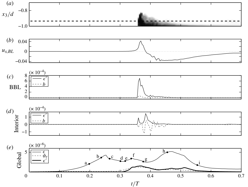
FIGURE 25. A comparison of local energetics to volume-integrated (global) energetics at x/L=0.83 (M3 in figure 22) for case 3. (a) Shows density as a function of depth and time using the same color scale as figure 2. (b) Shows the along-slope velocity at the boundary layer measurement location u_{s,BL} (in \text{m s}^{-1} ) as a function of time. (c,d) Local turbulent dissipation \epsilon' and buoyancy flux b , both in \text{m}^2 \text{s}^{-3} , in the BBL region (c) and the interior region (d). The vertical location of the interior measurement is shown by a dotted line in (a). (e) Volume-integrated (global) dissipation \epsilon , effective mixing rate \phi_e , and turbulent dissipation \int_V \epsilon' dV , all divided by the volume of the sloping region of the domain to give units of \text{m}^2 \text{s}^{-3} . Dots labelled a–i correspond to time snapshots from figures 2 and 6.
