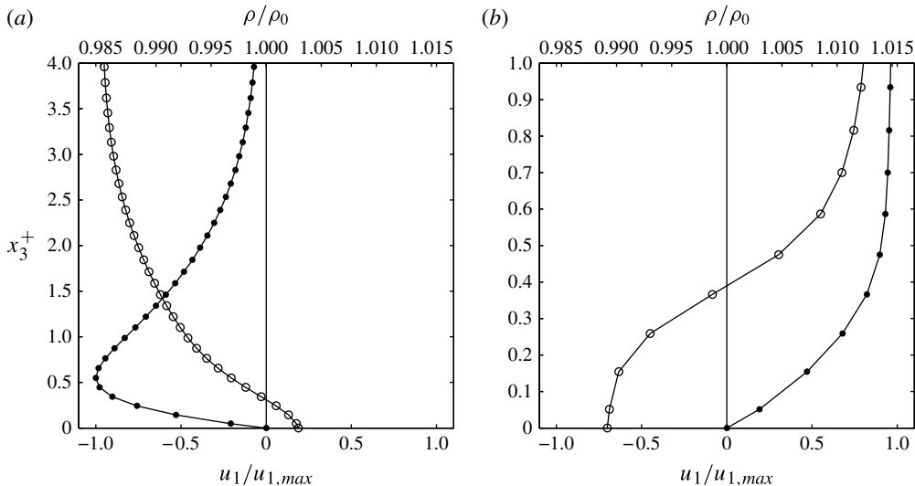
FIGURE 11. Vertical ( x_3 ) profiles of laterally-averaged horizontal velocity u_1 (●) and density \rho/\rho_0 (○). (a) A vertical profile corresponding to section A–A′ in figure 13(a). (b) A vertical profile corresponding to section E_2 – E'_2 (through the nose of the upslope surge) in figure 13(e). In both plots, u_1 is normalized by the maximum value over the full profile, and the vertical coordinate is shown in wall units x_3^+ = x_3/\delta_S measured upward from the bottom. Note the difference in the range of the vertical axes.
