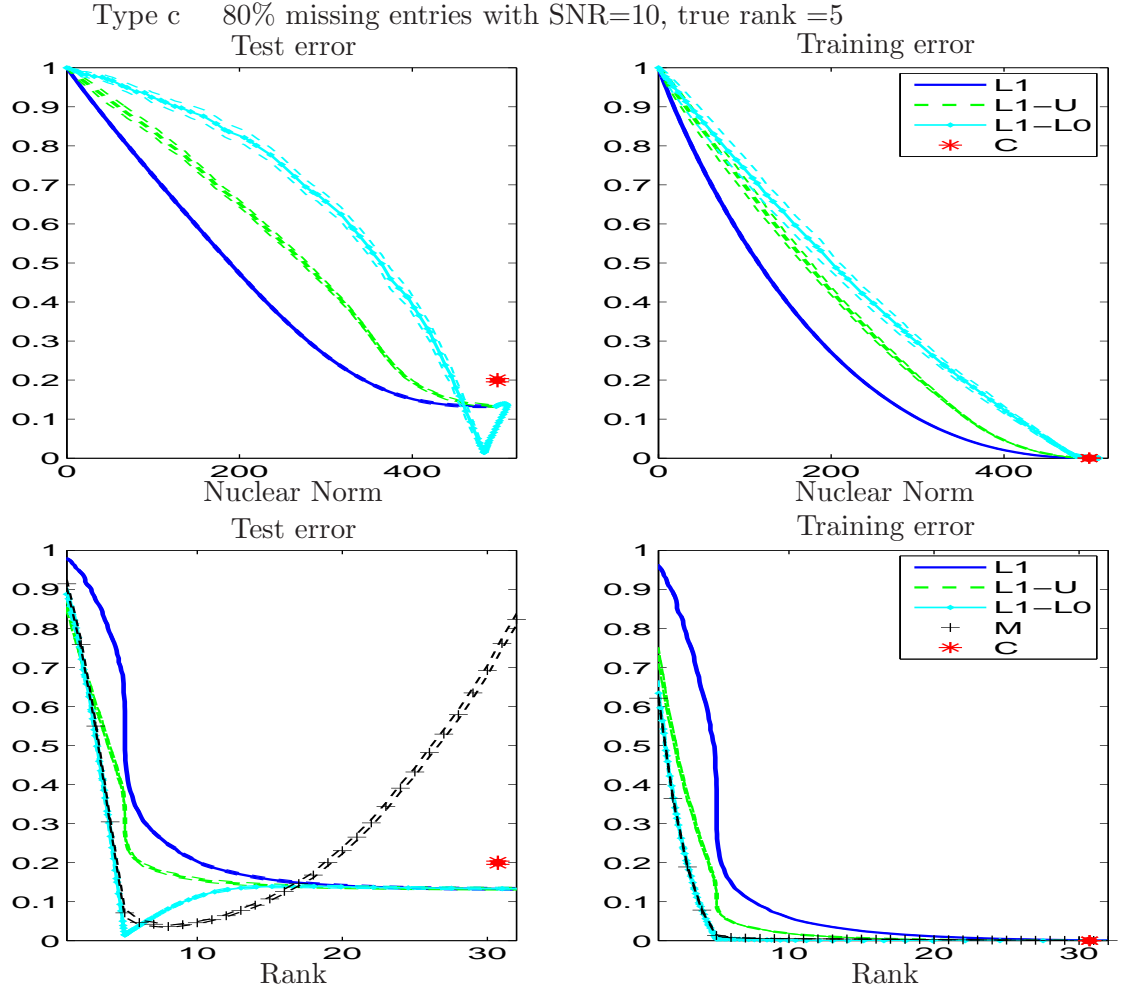
Figure 3: When the noise is low, HARD-IMPUTE can improve its performance. It gets the correct rank whereas OPTSPACE overestimates it. HARD-IMPUTE performs the best here wrt prediction error, followed by OPTSPACE. The latter does better than SOFT-IMPUTE. The noise here is low, still the SVT recovers a matrix with high rank approximately 30 and has poor prediction error as well. The test error of the SVT is found to be different from the limiting solution of SOFT-IMPUTE, though the former is allowed to run for 1000 iterations for convergence. This suggests that for small fluctuations of the objective criteria (11,2) around the minima the estimated “optimal solution” is not robust.
