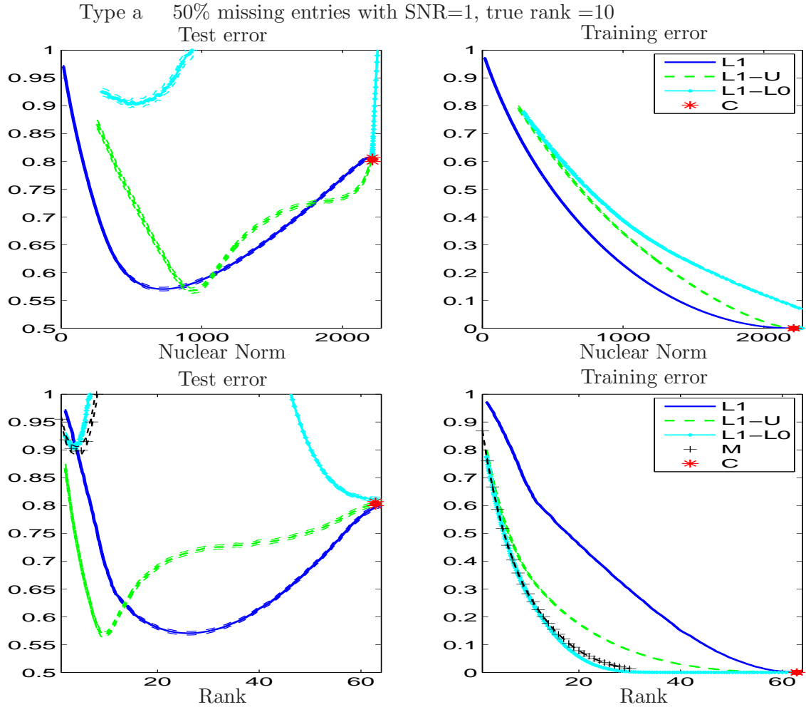
Figure 1: L1: solution for SOFT-IMPUTE; L1-U: Post processing after SOFT-IMPUTE; L1-L0 HARD-IMPUTE applied to L1-U; C : SVT algorithm; M: OPTSPACE algorithm. Both SOFT-IMPUTE and PP-SI perform well (prediction error) in the presence of noise. The latter estimates the actual rank of the matrix. Both the PP-SI and HARD-IMPUTE perform better than SOFT-IMPUTE in training error for the same rank or nuclear norm. HARD-IMPUTE and OPTSPACE perform poorly in prediction error. SVT algorithm does very poorly in prediction error, confirming our claim that (4) causes overfitting — it recovers a matrix with high nuclear norm and rank > 60 where the true rank is only 10. Values of test error larger than one are not shown in the figure. OPTSPACE is evaluated for a series of ranks \leq 30 .
