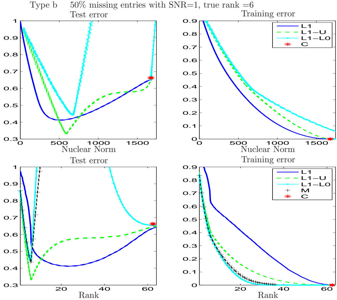
Figure 2: PP-SI does the best in prediction error, closely followed by SOFT-IMPUTE. Both HARD-IMPUTE, OPTSPACE have poor prediction error apart from near the true rank of the matrix ie 6 where they show reasonable performance. SVT algorithm does very poorly in prediction error — it recovers a matrix with high nuclear norm and rank > 60 where the true rank is only 6. OPTSPACE is evaluated for a series of ranks \leq 35 .
