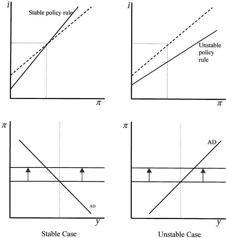
Fig. 1. Illustration of stable versus unstable monetary policy rules. On the left the slope of the policy rule is greater than one and aggregate demand is negatively sloped, causing y to fall following an inflation shock, which is stabilizing. On the right the slope of the policy rule is less than one and aggregate demand is upward sloping, which is destabilizing.
