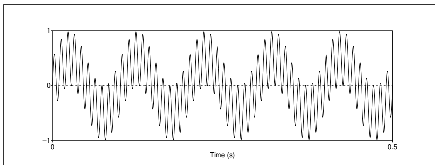
Figure H.15 A waveform that is the sum of two sine waveforms, one of frequency 10 Hz (note five repetitions in the half-second window) and one of frequency 100 Hz, both of amplitude 1.
