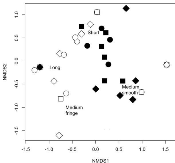
Fig 2 – Functional NMDS ordination based on hyphal exploration type for soil cores sampled across the edge-interior of three Pinus muricata tree islands. Each point represents a single soil core. Points closer together have more similar composition of hyphal exploration types. Symbols denote different tree islands (Circle = 1, Square = 2, Diamond = 3) and black and white colors represent interior and edge samples, respectively. Text indicates the portion of the ordination with which each hyphal exploration type was most associated. Despite the fact that there were no significant differences in species composition between edge and interior samples, functional composition varied significantly with sampling location.
