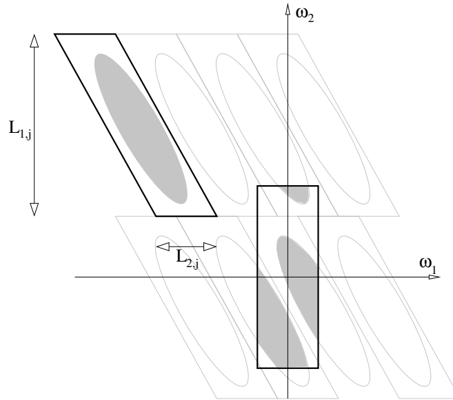
FIG. 3. Wrapping data, initially inside a parallelogram, into a rectangle by periodicity. The angle \theta is here in the range (\pi/4, 3\pi/4) . The black parallelogram is the tile \mathcal{P}_{j,\ell} which contains the frequency support of the curvelet, whereas the grey parallelograms are the replicas resulting from periodization. The rectangle is centered at the origin. The wrapped ellipse appears “broken into pieces,” but as we shall see, this is not an issue in the periodic rectangle, where the opposite edges are identified.
