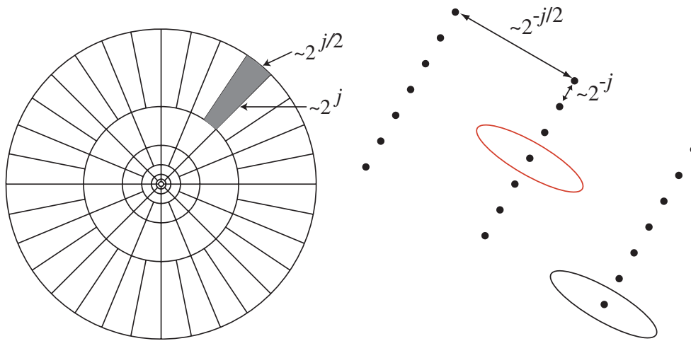
FIG. 1. Curvelet tiling of space and frequency. The image on the left represents the induced tiling of the frequency plane. In Fourier space, curvelets are supported near a “parabolic” wedge, and the shaded area represents such a generic wedge. The image on the right schematically represents the spatial Cartesian grid associated with a given scale and orientation.
