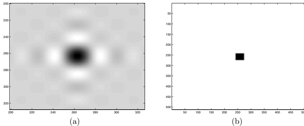
FIG. 9. At the coarsest level, curvelets are nondirectional and are Meyer scaling functions. (a) Spatial side. The color map is as follows: white is most negative, zero corresponds to some tone of grey, and black is most positive. (b) Frequency side (modulus of the Fourier transform). The level of grey indicates values from zero (white) to one (black).
