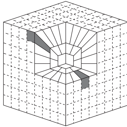
FIG. 8. The dyadic-parabolic frequency tiling in three dimensions. Curvelets are supported near the grey regions.
