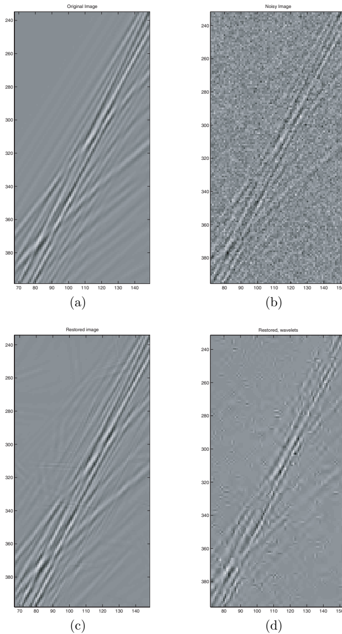
FIG. 14. Image denoising using curvelets. (a) The original image (zoom). (b) Noisy image (Gaussian white noise with \sigma = 10\% of the maximum intensity), PSNR = 20.0 dB. (c) Denoised image using curvelets, PSNR = 37.6 dB. (d) Denoised image using wavelets, PSNR = 30.8 dB.
