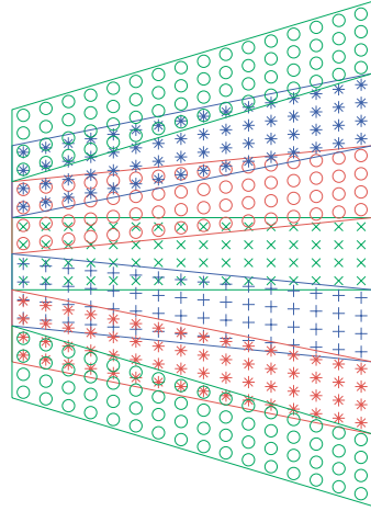
FIG. 4. This figure illustrates the sampling within each parallelepipedal region according to an equispaced grid aligned with the axes of the parallelogram. There are as many parallelograms as there are angles \theta_\ell \in [-\pi/4, \pi/4] .
