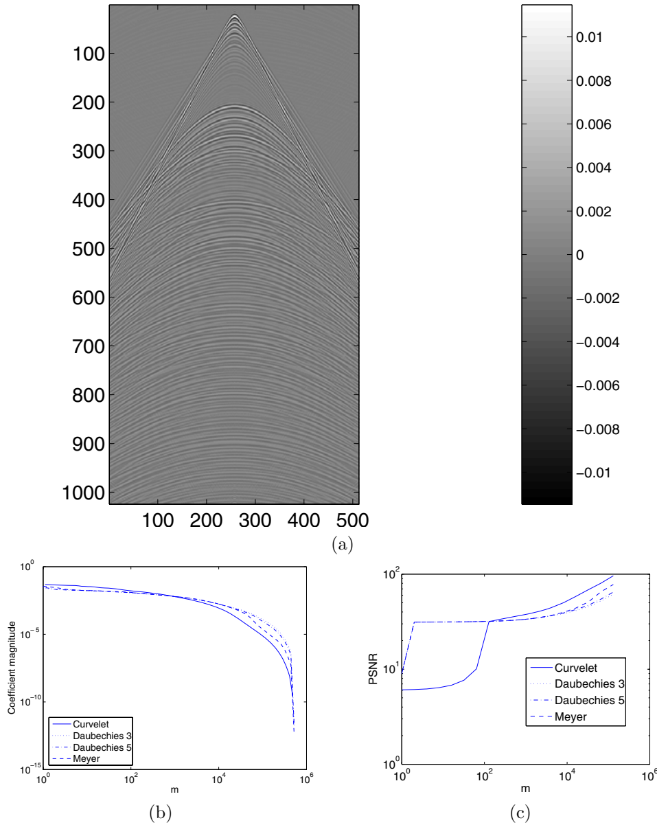
FIG. 13. Sparsity analysis of the curvelet and wavelet representations of a seismogram. (a) Synthetic seismogram corresponding to the acoustic response of a 1D layered medium to a point source, courtesy of Eric Verschuur and Felix Herrmann. The x-axis is the offset from the source, and the y-axis is time. (b) Decay of the coefficients. (c) Partial reconstruction error, measured in PSNR.
