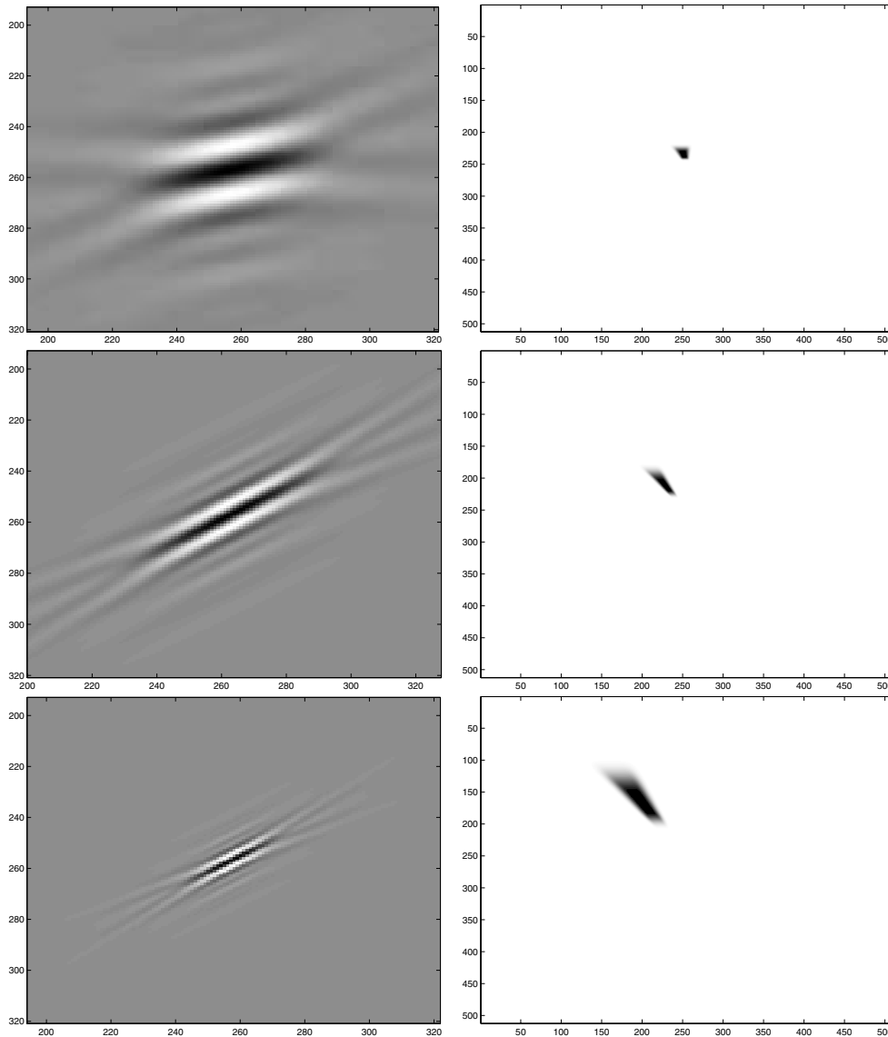
FIG. 10. Curvelets at increasingly fine scales. The left panels represent curvelets (real part) in the spatial domain (as functions of the spatial variable x ). The right panels show the modulus of the Fourier transform (as functions of the frequency variable \omega ). The color map is the same as in Figure 9.
