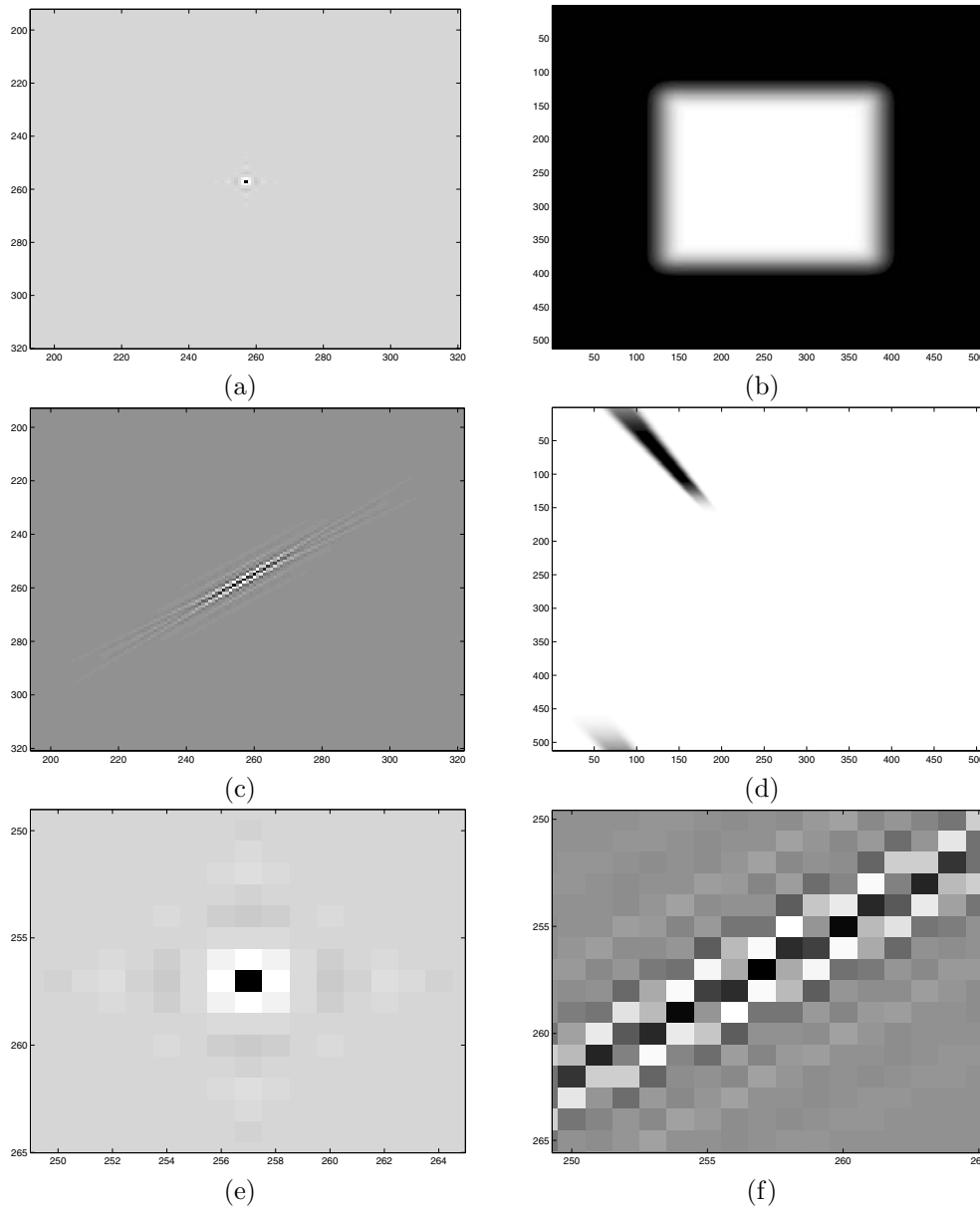
FIG. 11. Wavelets and curvelets at the finest scale. Meyer wavelet in space (a) and frequency (b). Undersampled curvelet in space (c) and frequency (d). (e) Zoom of (a). (f) Zoom of (c).
