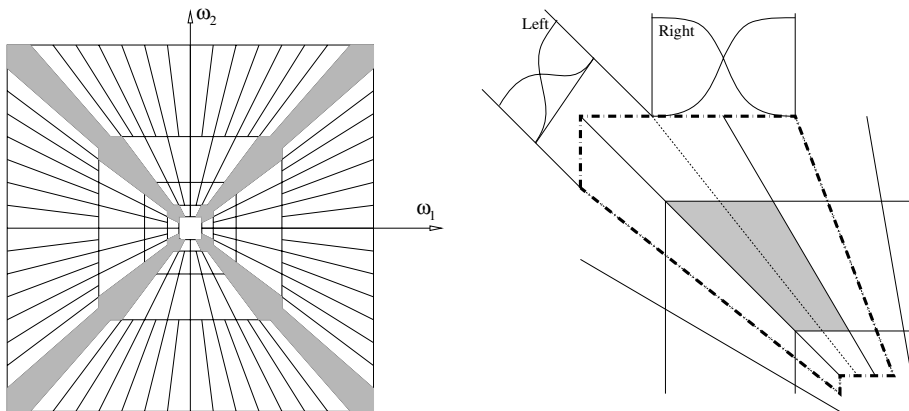
FIG. 7. Left: The corner wedges appear in grey. Right: Detail of the construction of a partition of unity over the junction between quadrants.
