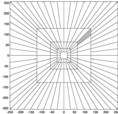
FIG. 2. The figure illustrates the basic digital tiling. The windows \tilde{U}_{j,\ell} smoothly localize the Fourier transform near the sheared wedges obeying the parabolic scaling. The shaded region represents one such typical wedge.
