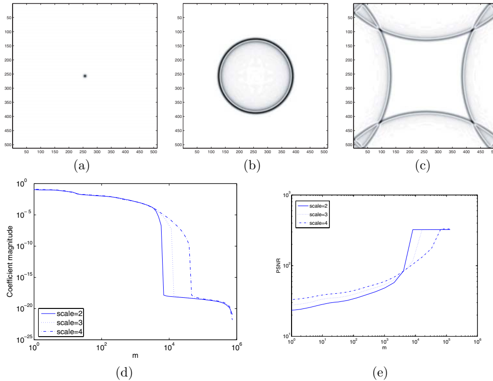
FIG. 15. Compression of the wavefield and of the solution operator to the wave equation with periodic boundary conditions. (a) The initial condition is a delta function located at the center of the domain. (b) Approximate solution at t = 0.25 . (c) Approximate solution at t = 0.75 . Both approximations use only 1.25% of nonzero curvelet coefficients. (d) Magnitude of the matrix entries (rearranged in descending order) of the solution operator E_t at t = 0.75 taken from three columns corresponding to three curvelets at various scales. (e) For the same three columns, truncation error obtained by keeping the m largest entries, measured in PSNR.
