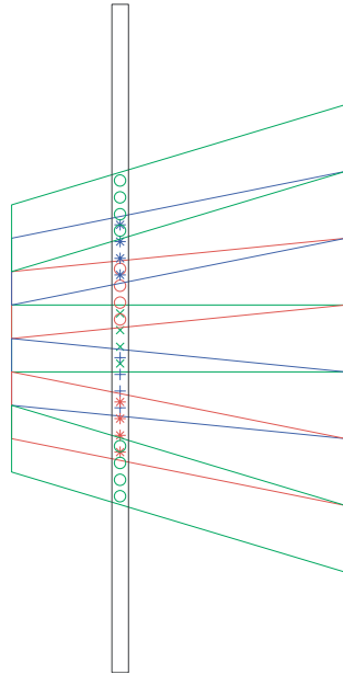
FIG. 5. This figure illustrates a key property of the USFFT version. The interpolation step is organized so that it is obtained by solving a sequence of 1D problems. For a fixed column, we need to resample a 1D trigonometric polynomial on the mesh shown here.
