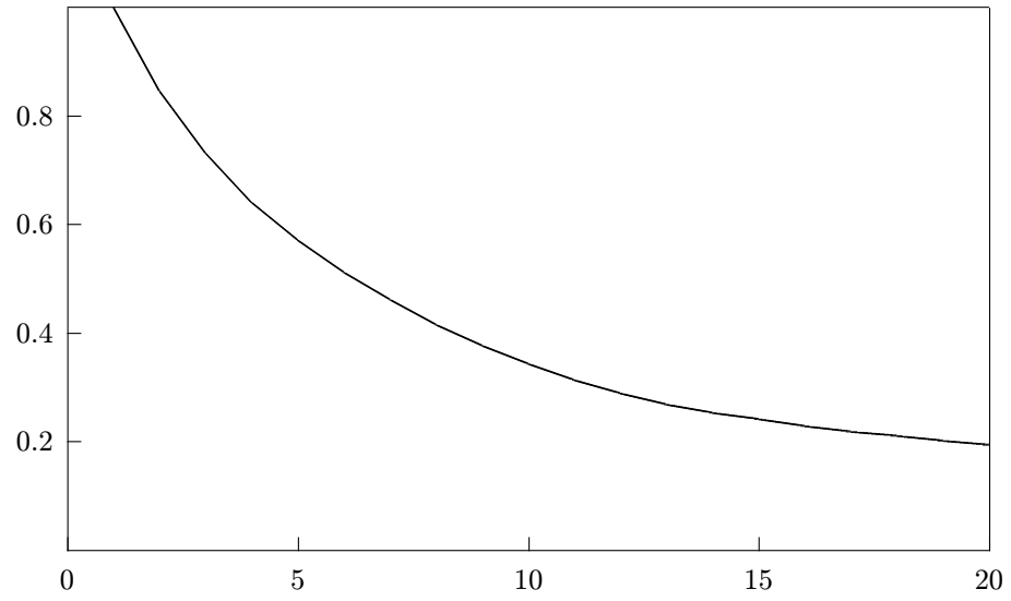
Figure 3: Variance Ratios.
